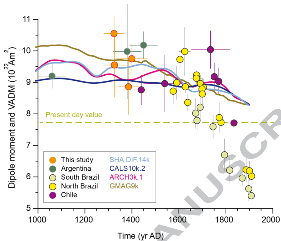
Figure 7. High-quality VADM values available for South America for the last 1000 years and comparison with different global dipole moment reconstructions (see text for further details).
