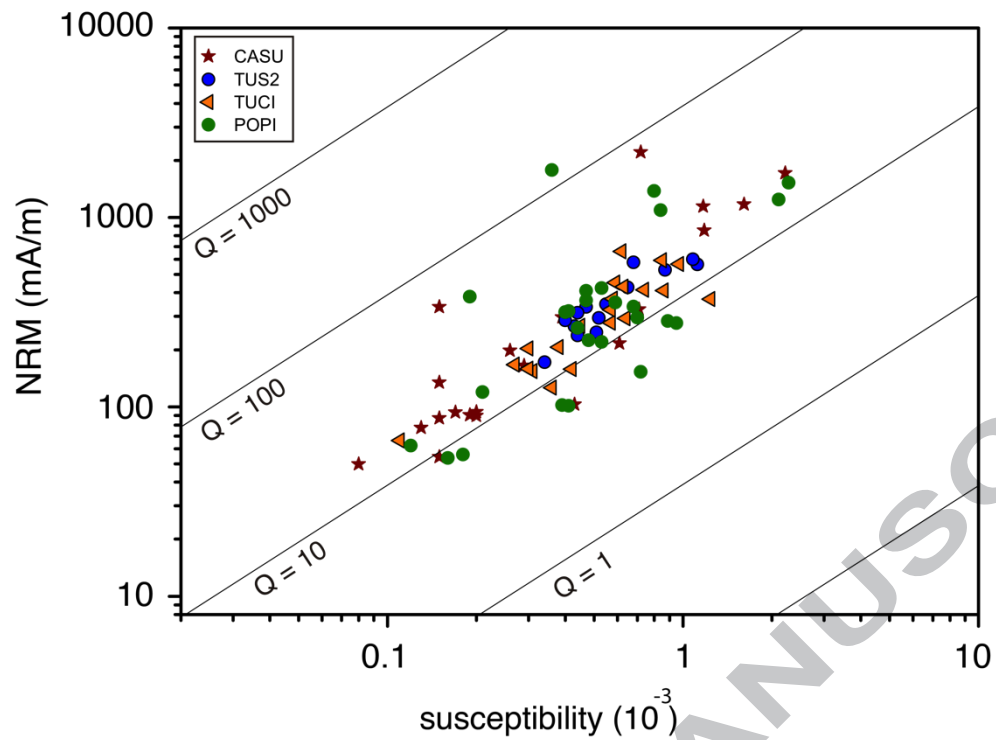
Figure 2. Intensity of the Natural Remanent Magnetization (NRM) versus bulk susceptibility ( 10^{-3} SI). Lines indicate constant Königsberger ratios ( Q ).
