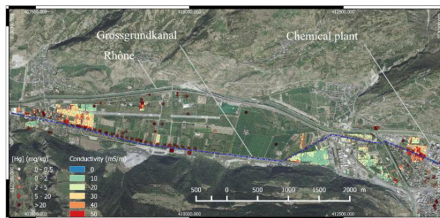
Fig. 1. EM conductivity and topsoil Hg concentration map.
