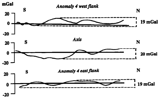
Fig. 6. Mantle Bouguer anomaly profiles along isochrons on the ridge axis and on the flanks at anomaly 4. Note the constant amplitude of anomalies between the axis and the flanks.
