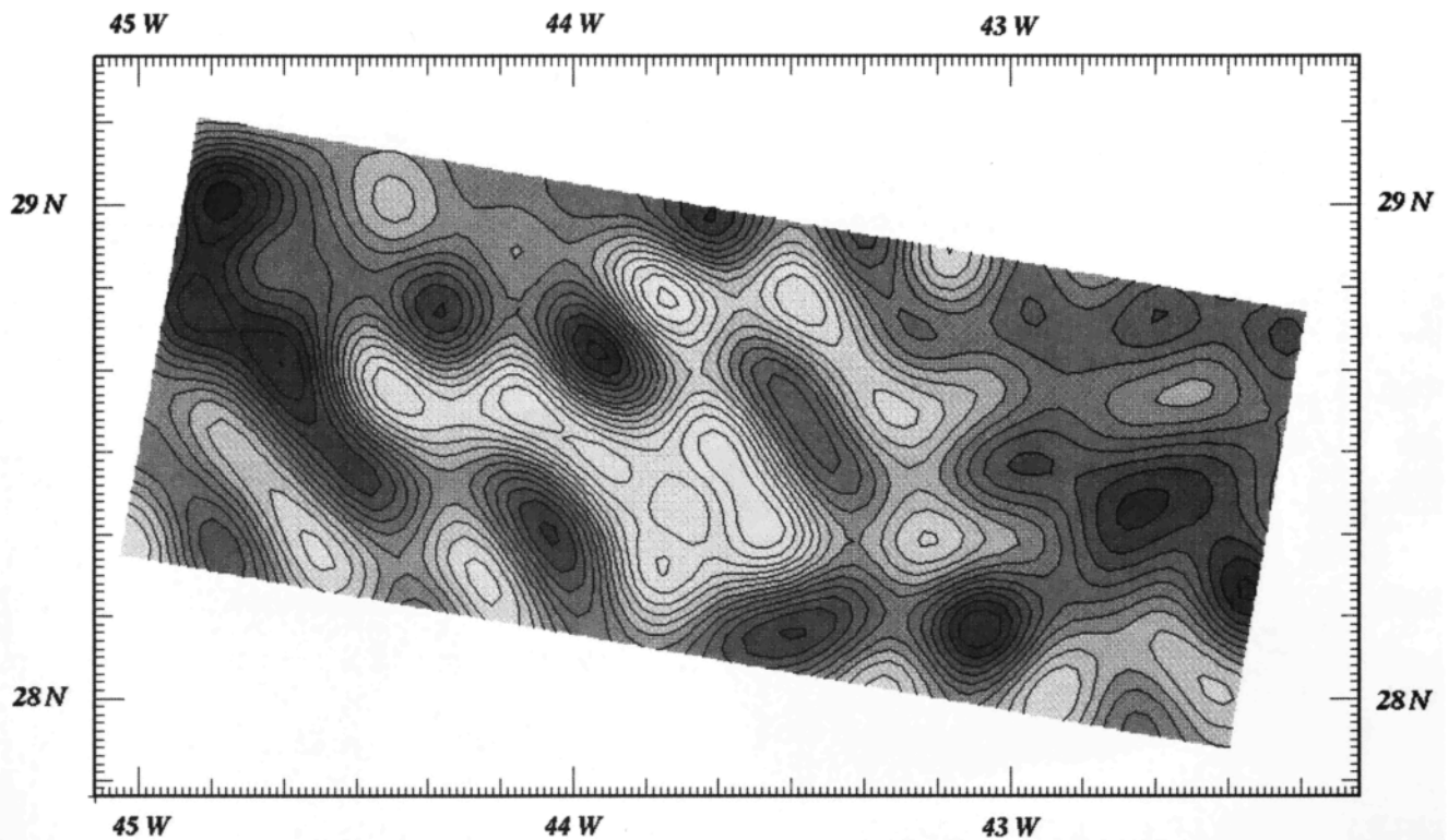
Fig. 7a. Map of variations in crustal thickness determined by downward continuation of the residual gravity anomalies to 8 km level. The contour interval is 200 m, and the values represent deviations from an assumed 5 km thick crust.
