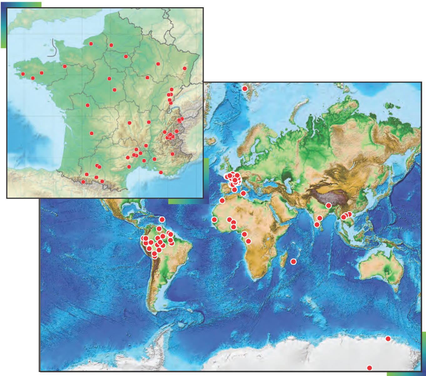
Fig. 5. World map of OZCAR instrumented sites. More than 60 instrumented sites (with scales ranging from the plot to the whole river catchment) are included in 21 observatories or observation services (not represented) funded and evaluated by diverse research agencies. All are monitoring parts of the critical zone.
