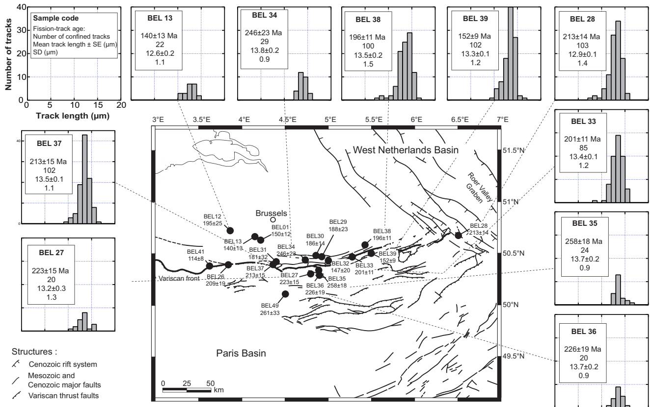
Fig. 4. Geographical distribution of the FT results of the northern Ardenne and Brabant Massifs. Histograms show confined track-length distributions: y-axis: frequency of tracks; x-axis: length in μm; text from the top: sample code; AFT age ± standard deviation; number of measured tracks; mean track length ± standard deviation (both in μm).
