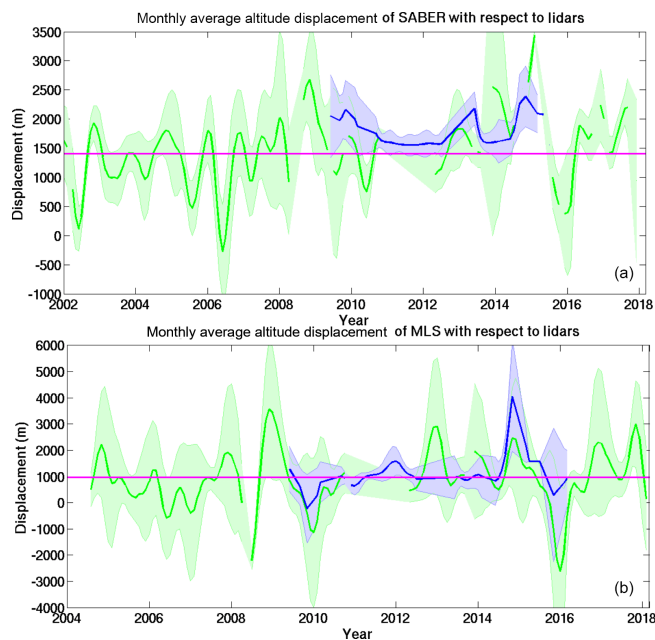
Figure 10. Panel (a) features the monthly average displacement of SABER measurements with respect to the OHP lidars (green for LTA and blue for \text{LiO}_3\text{S} ). The standard deviation is given as the shaded area. The mean offset (magenta) is 1446 m with a standard error of 49 m. Panel (b) shows the same analysis with the monthly average MLS displacement. The mean value is 911 m with a standard error of 90 m.
