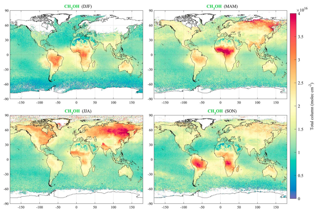
Figure 10. Seasonal means (on a 0.5 \times 0.5^\circ grid) of the ANNI- \text{CH}_3\text{OH} total columns from the a.m. (morning overpasses) IASI measurements over the year 2011. The same distributions, but produced from the p.m. (evening overpasses) IASI observations, are shown in Figure S9 in the supporting information. ANNI = Artificial Neural Network for IASI; IASI = Infrared Atmospheric Sounding Interferometer.
