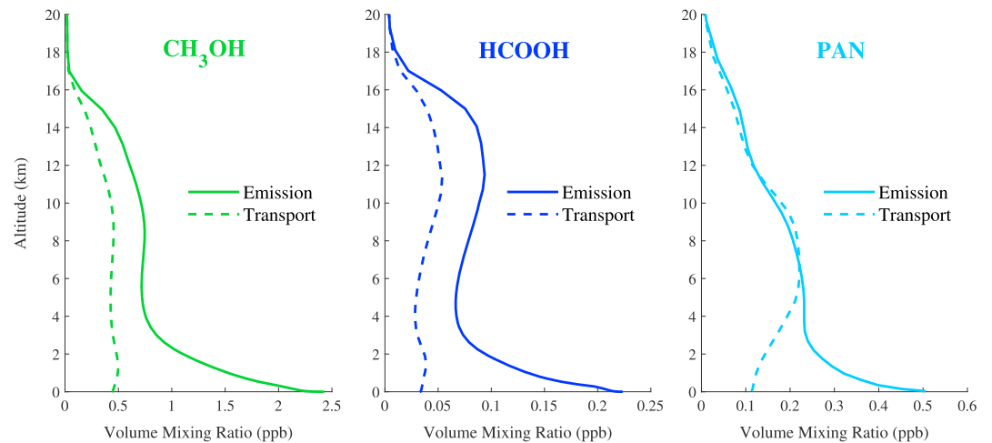
Figure 4. Vertical concentration profiles of \text{CH}_3\text{OH} , \text{HCOOH} , and PAN, derived from global model simulations, which are used to perform the forward simulations of Infrared Atmospheric Sounding Interferometer spectra for the neural network synthetic training sets. For each target species, an emission and a transport profile (in solid and dashed lines, respectively) have been produced (see section 3.1). PAN = peroxyacetyl nitrate.
