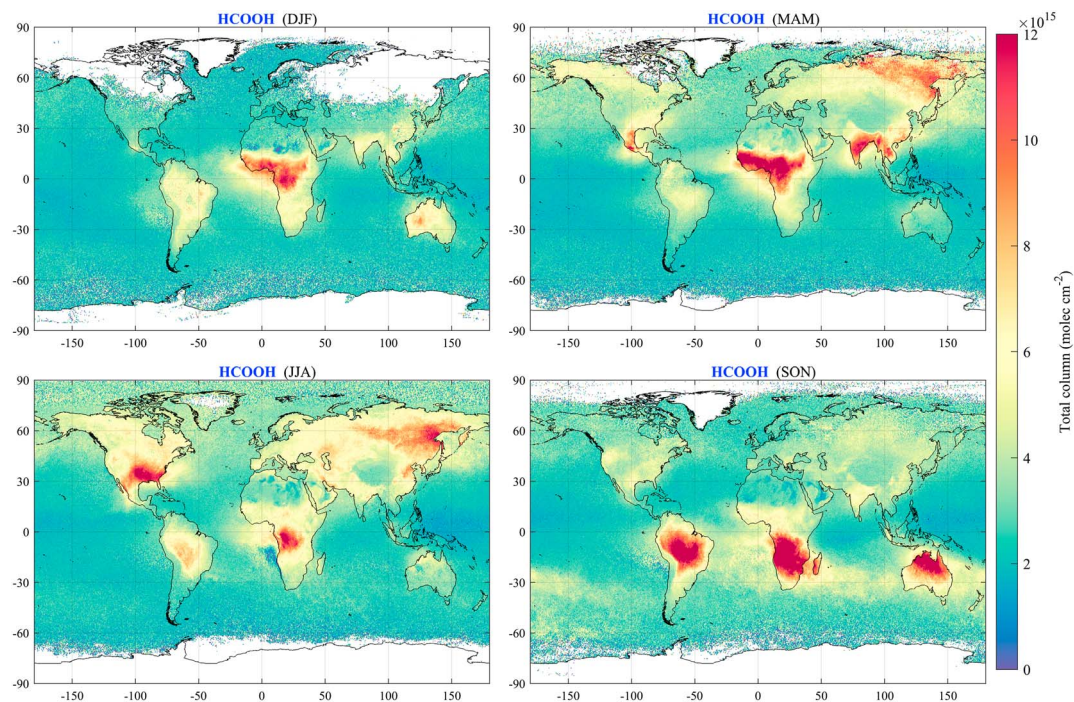
Figure 11. Seasonal means (on a 0.5 \times 0.5^\circ grid) of the ANNI-HCOOH total columns from the a.m. (morning overpasses) IASI measurements over the year 2011. The same distributions, but produced from the p.m. (evening overpasses) IASI observations, are shown in Figure S10 in the supporting information. ANNI = Artificial Neural Network for IASI; IASI = Infrared Atmospheric Sounding Interferometer.
