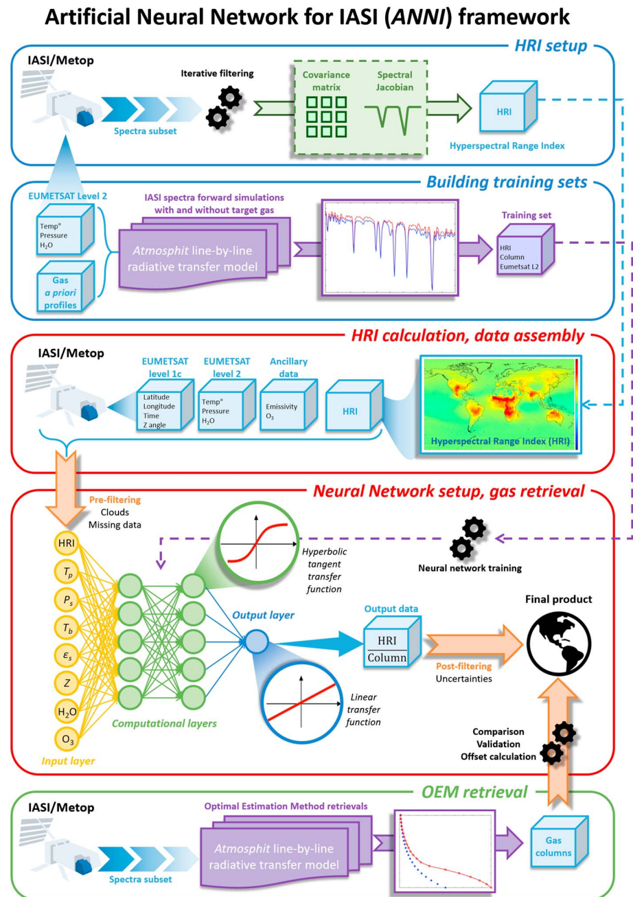
Figure 1. Conceptual flowchart of the ANNI (Artificial Neural Network for IASI) retrieval method of trace gases. IASI = Infrared Atmospheric Sounding Interferometer.
