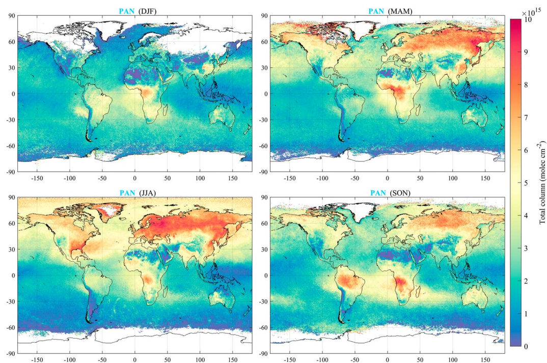
Figure 12. Seasonal means (on a 0.5 \times 0.5^\circ grid) of the ANNI-PAN total columns from the a.m. (morning overpasses) IASI measurements over the year 2011. The same distributions, but produced from the p.m. (evening overpasses) IASI observations, are shown in Figure S11 in the supporting information. ANNI = Artificial Neural Network for IASI; IASI = Infrared Atmospheric Sounding Interferometer; PAN = peroxyacetyl nitrate.
