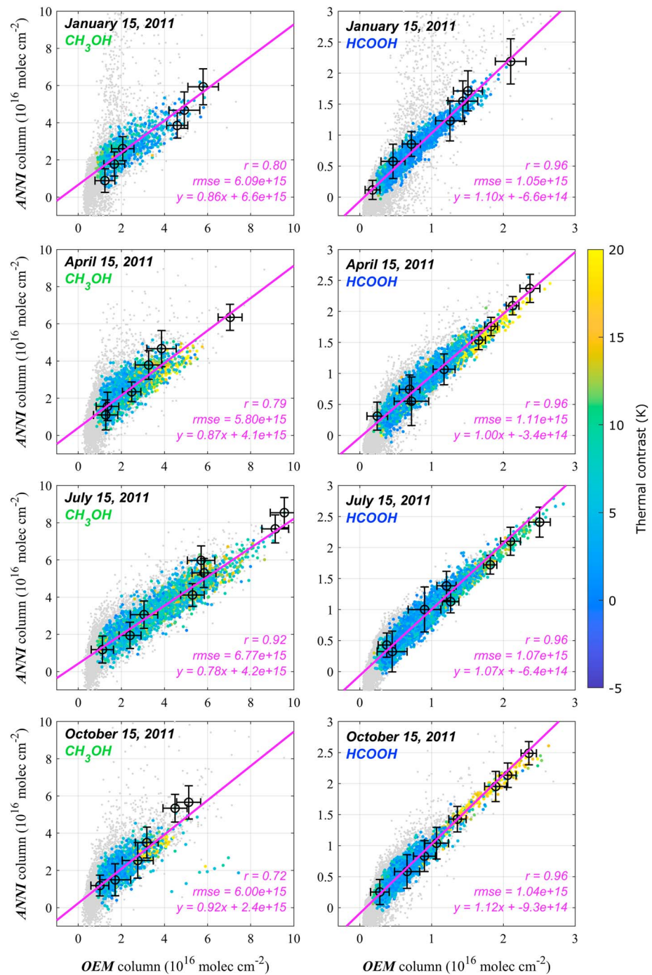
Figure 7. Comparison between \text{CH}_3\text{OH} and \text{HCOOH} total columns from the ANNI processing (y axis) and retrieved with an OEM (x axis). Pixels are colored by thermal contrast. The spectra have been selected from 4 days of 2011 over specific regions (see Figure S5). Postfiltering has been applied to both data sets (see section 4.1). The measurements filtered out of the comparison are depicted as gray dots. The linear regression, root-mean-square error ( rmse ) and coefficient of correlation ( r ) between the two data sets are given in magenta. The ANNI and OEM uncertainties for random measurements are also indicated for selected measurements (in black). The present comparison only includes measurements performed over land. Figure S6 illustrates the same comparison for the observations over oceans. ANNI = Artificial Neural Network for IASI; IASI = Infrared Atmospheric Sounding Interferometer; OEM = optimal estimation method.
