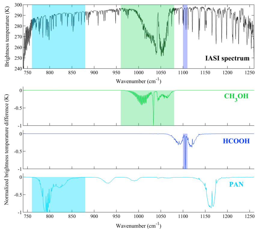
Figure 2. Typical IASI spectrum (displayed in brightness temperature) in the 750–1,250 \text{cm}^{-1} spectral range (upper frame), and the Jacobians K of the \text{CH}_3\text{OH} , \text{HCOOH} , and PAN spectral absorptions used for the calculation of the HRI (lower frames). The spectral ranges selected for the retrieval of each species are illustrated in colored rectangles. In the lower frames, the brightness temperatures were normalized to have a minimum value of -1 for visibility purposes. The Jacobians K have been produced by the line-by-line radiative transfer model Atmosphit (Coheur et al., 2005) for a standard atmosphere. The IASI spectrum illustrated here has been recorded at 33.21°N, 89.22°W, on 15 July 2011 (~9:30 UTC), at a viewing angle Z of 37.09°. IASI = Infrared Atmospheric Sounding Interferometer; PAN = peroxyacetyl nitrate.
