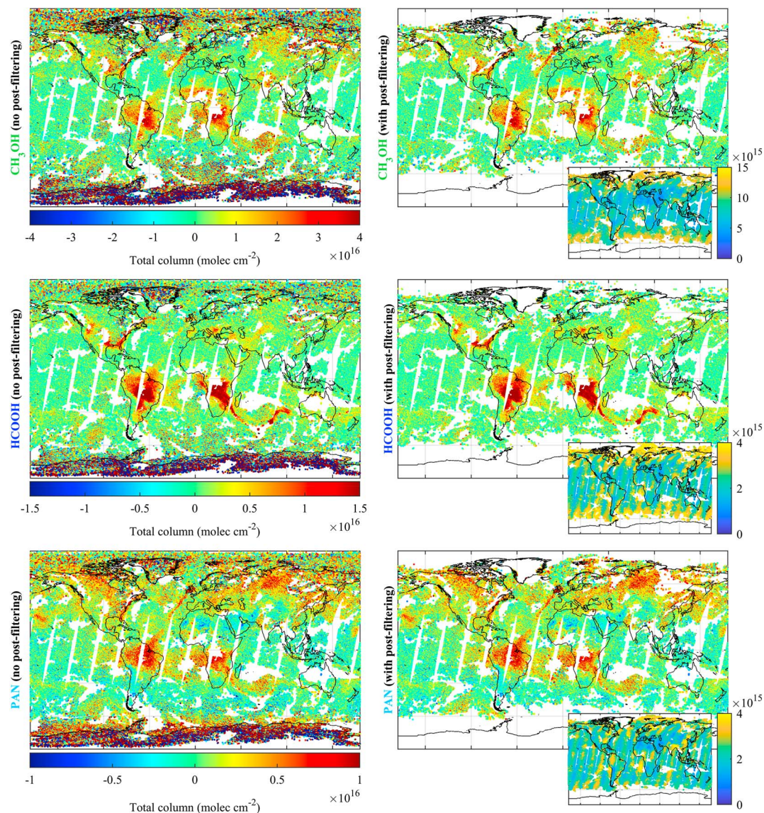
Figure 6. Impact of the postfiltering of the NN-derived total columns on the global \text{CH}_3\text{OH} , \text{HCOOH} , and PAN distributions. The left and right frames show the unfiltered and postfiltered distributions, respectively (see section 4.1). The gas total columns are retrieved from the a.m. (morning overpasses) IASI observations performed on 9 September 2011. The blank spaces on the left frames are due to gaps between the successive satellite orbits (within the Tropics) or to the prefilter excluding the cloudy scenes. The insets show the individual retrieved column uncertainties in molecules per square centimeter (see section 4.1).
