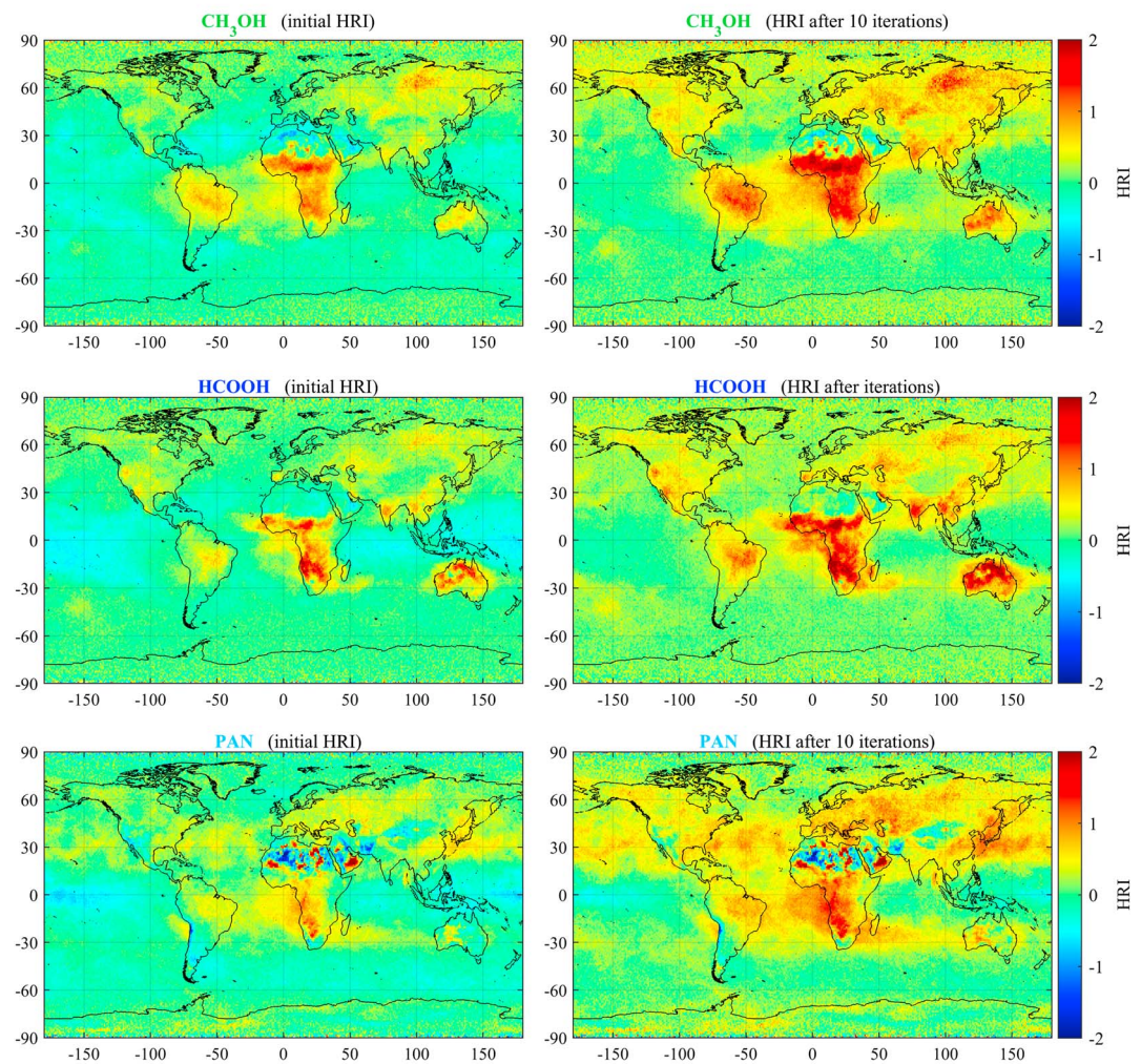
Figure 3. Examples of annual mean HRI for CH 3 OH, HCOOH, and PAN over 2013, calculated from a whole set of IASI spectra without filtering (left frames), or derived from a spectra subset after 10 iterations of the filtering procedure (right frames) (see section 2.2). Note the emissivity affecting the PAN-HRI over deserts; these are corrected before ingestion into the NN. HRI = hyperspectral range index; IASI = Infrared Atmospheric Sounding Interferometer.
