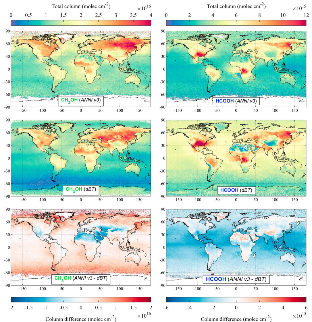
Figure 8. Comparison between the ANNI-CH 3 OH and ANNI-HCOOH products, and the global distributions obtained from IASI with retrieval methods based on dBT (Razavi et al., 2011, for CH 3 OH and Pommier et al., 2016, for HCOOH), over the boreal summer (June–August) of the year 2011. The comparison for the boreal winter (December–February) is shown in Figure S8 in the supporting information.
