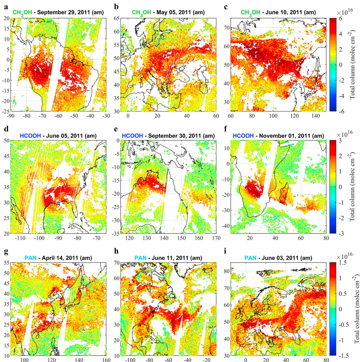
Figure 9. \text{CH}_3\text{OH} , \text{HCOOH} , and PAN total column distributions retrieved over areas of interest with the ANNI method from 1 day of a.m. (morning overpasses) IASI observations. Each colored dot corresponds to an individual IASI measurement. The blank spaces are due to gaps between the successive satellite orbits (within the Tropics) or to data filtered out because of clouds or postfiltering (bad retrievals). ANNI = Artificial Neural Network for IASI; IASI = Infrared Atmospheric Sounding Interferometer; PAN = peroxyacetyl nitrate.
