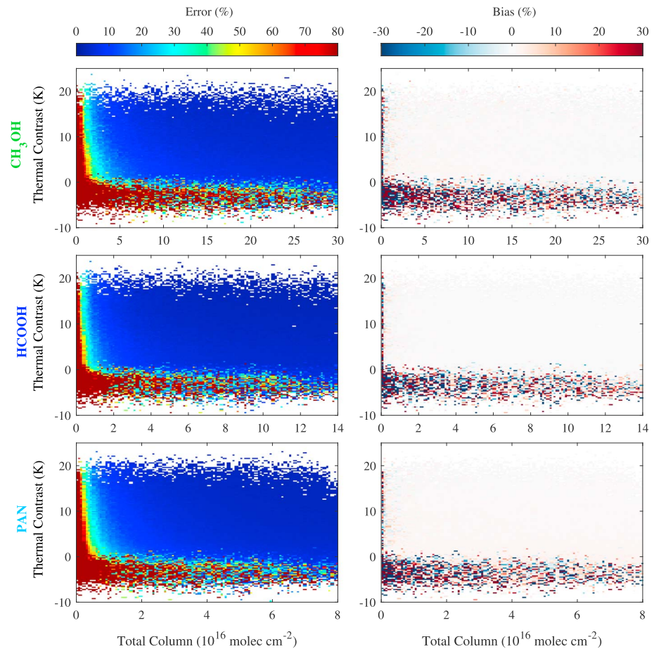
Figure 5. Training performance of the neural network (NN) trained with the emission profile of the target species. The relative error (left frames) and bias (right frames) of the NN-derived gas total columns over the actual columns are displayed as a function of the thermal contrast and gas vertical abundance. To be representative for the real Infrared Atmospheric Sounding Interferometer observations, random noise has been added to all variables used in input of the NN. The same evaluation, but for the transport-NN, is shown in Figure S3 in the supporting information. PAN = peroxyacetyl nitrate.
