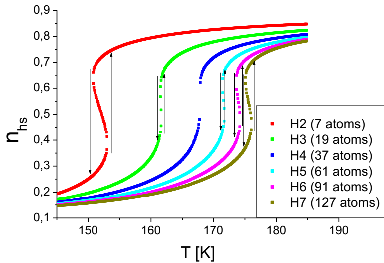
Figure 3 : The simulated thermal behavior of the total high spin (HS) fraction, N_{hs}(T) , for different system sizes from H2 (7 atoms) to H7 (127 atoms). The computational parameters are: \Delta/k_B = 1200 K, G/k_B = 170 K, J/k_B = 15 K, L/k_B = 125 K, \ln(g) = 6.5 .
