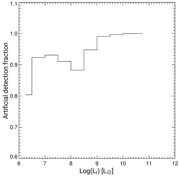
Fig. A.3. Artificial detection fraction as a function of r -band luminosity for our artificial H I masses.
