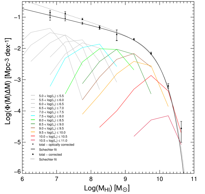
Fig. 9. Reconstructed HIMF per luminosity bin, \log(\Phi(M)\Delta M) in units of \text{Mpc}^{-3} \text{dex}^{-1} , as a function of H I mass in each luminosity bin, shown as a set of colored and gray curves. We recreated a plot similar to Fig. 5 with artificial H I mass distributions for luminosity bins below \log(L_r) = 7.75 shown in gray. We omit the uncertainty regions on each luminosity bin for viewing clarity. Uncertainties for the colored bins are the same as those in Fig. 5 and uncertainties for the gray bins are given in Table 2. Two reconstructed HIMFs are shown: the one based on the optically corrected BLF (which ignores the change in detection fraction with luminosity) is denoted by dots with a solid Schechter fit line, the other based on the corrected BLF (which takes this change into account) is denoted by triangles with a dotted Schechter fit line.
