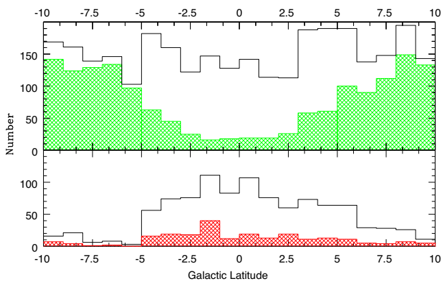
Figure 2. Histogram of the 2MASX ZoA bright galaxies with |b| < 10^\circ for the NRT visibility range \delta > -40^\circ . Top panel: the black histograms demarcate all 2MZoAG galaxies and green are the ones with redshifts in 2MRS (Huchra et al. 2012) complemented by the low-latitude zcat compilation. Bottom panel: the Nançay target sample (all observed), where the red histogram highlights the HI detections (see Section 4).
