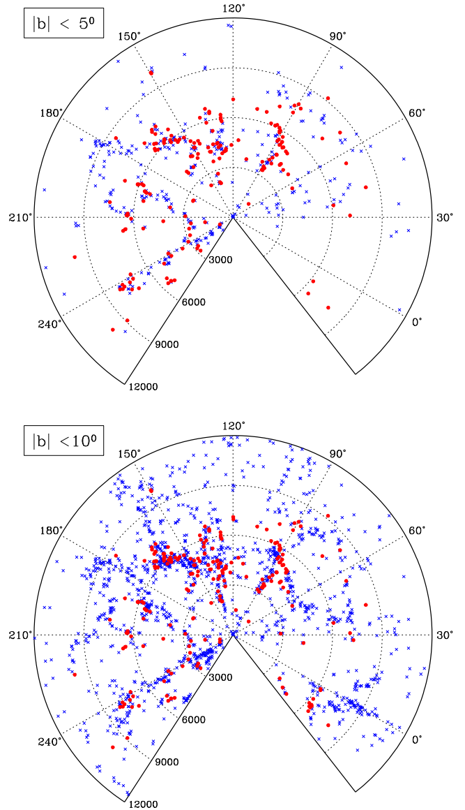
Figure 12. Redshift wedge out to V_{\text{hel}} < 12000\text{ km s}^{-1} centred on the longitude range of the Nançay 2MZOAG survey. Red dots represent NRT HI detections, and blue crosses 2MASX galaxies with prior redshift measurements. The top panel displays the inner ZoA ( |b| < 5^\circ ) and the bottom panel the full width of the 2MZOAG survey ( |b| < 10^\circ ). The most prominent new ZoA feature is the wall-like structure that forms part of the PPS (running from about \ell \sim 125^\circ at 4500\text{ km s}^{-1} to 165^\circ and 6500\text{ km s}^{-1} ). The latter includes the new filament around \ell \sim 165^\circ in which the 3C 129 cluster is embedded.
