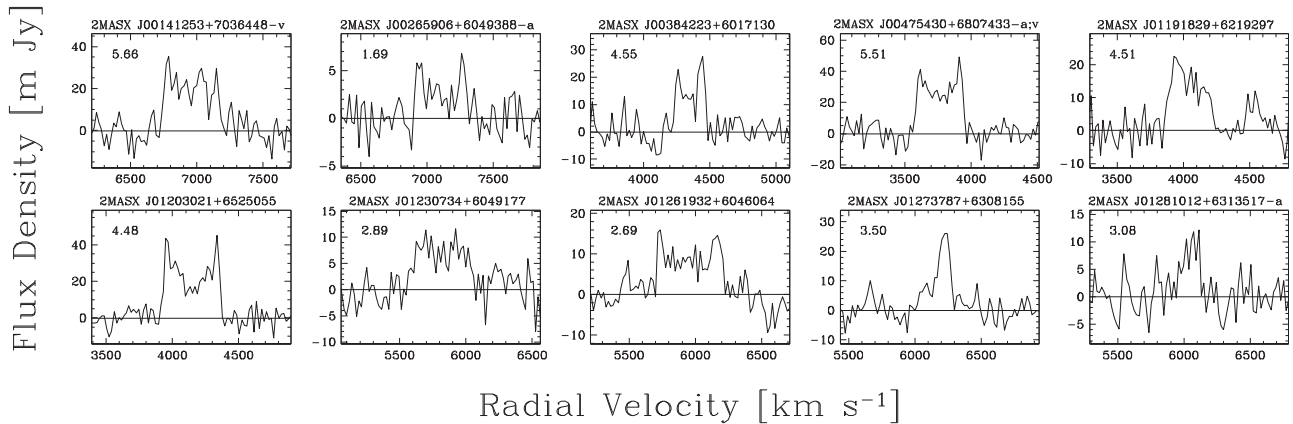
Figure 4. Example of the first two rows of the Nançay 21 cm HI line spectra of detected galaxies. The velocity resolution is 18 \text{ km s}^{-1} . The full figure of all detections (Tables 1 and 2 combined) is available online as Fig. A1.
