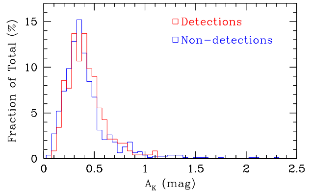
Figure 3. Distribution of extinction A_K of the in HI-detected galaxies (red; N = 230 ) versus the non-detections (blue; N = 773 ), both as a fraction of their respective total. As expected, the detection rate shows no dependence on foreground extinction.
