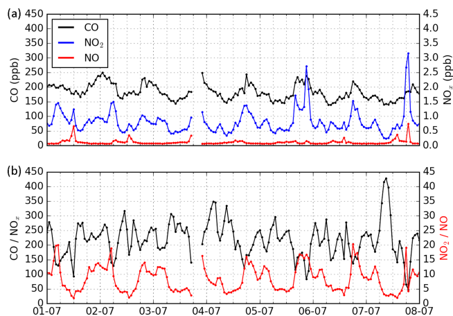
Figure 5. Time series of (a) carbon monoxide (CO), nitrogen dioxide ( \text{NO}_2 ), and nitrogen monoxide (NO) hourly concentration averages (ppb) observed at Savè (Benin) for the period of 1–7 July 2016 and (b) of the ratios \text{CO}/\text{NO}_x (in black) and \text{NO}_2/\text{NO} (in red). The vertical dashed lines indicate periods of 6 h starting at 00:00 UTC.
