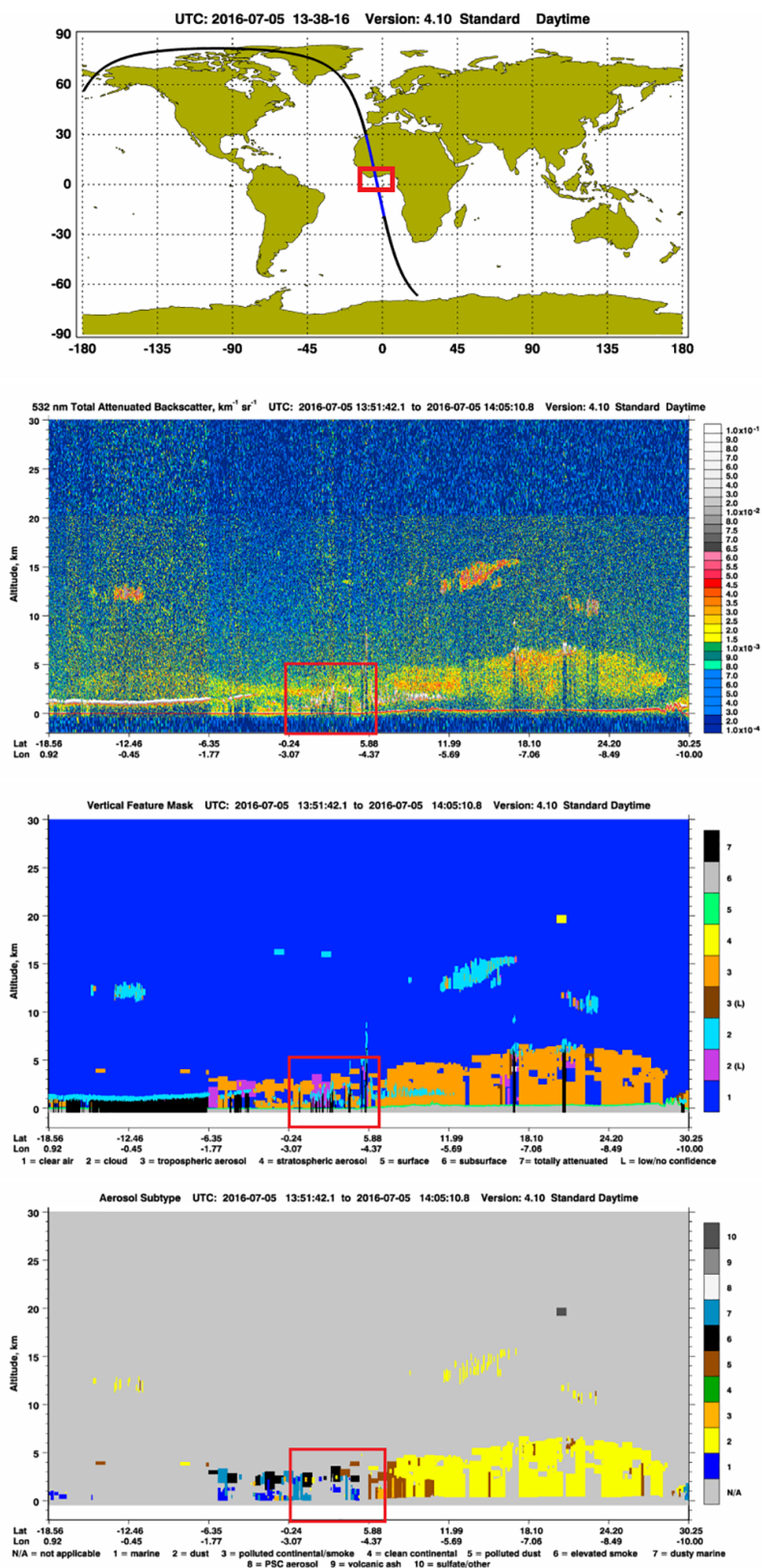
Figure A2. Space lidar CALIPSO data on board the CALIOP platform on 5 July 2016 with the orbit track location, the vertical profile of the total attenuated backscatter, the vertical feature mask, and the aerosol subtype. The modeling domain is the red box (data are available at https://www-calipso.larc.nasa.gov/ , last access: 10 January 2019).
