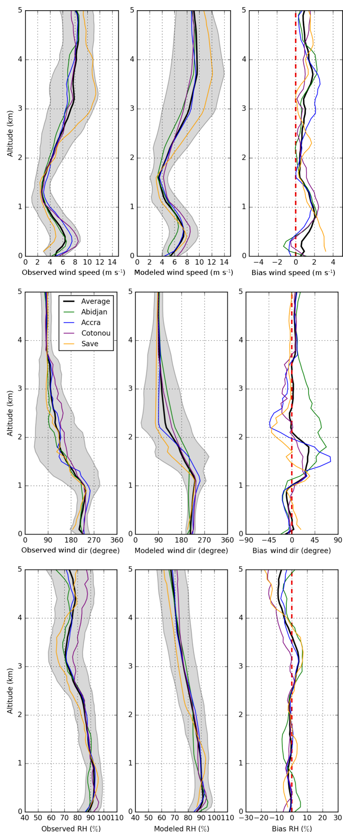
Figure 3. Observed and modeled mean vertical profiles of wind speed ( \text{m s}^{-1} ) and direction ( 360^\circ circle with 0 and 360^\circ is the north and 90^\circ is the east) and relative humidity (RH in %) averaged for all profiles over the period of 1–7 July 2016 at Abidjan in Côte d’Ivoire (green line), Accra in Ghana (blue line), Cotonou in Benin (purple line), and Savè in Benin (orange line). The mean and standard deviation at the four locations are represented by the black line and the gray shading. WRF-derived variables are interpolated to the radiosonde positions. The right panel presents the (mod–obs) mean vertical bias of each location and of the average of the four locations.
