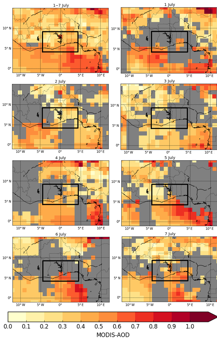
Figure A1. MODIS AOD daily average of two products acquired by Aqua and Terra (the combined Dark Target and Deep Blue MYD08-D3 and MOD08-D3 products, respectively) over the 1–7 July 2016 period (top left) and over each day of the period. Data excluded by the cloud screening process are in gray. The modeling domain is presented by the black square.
