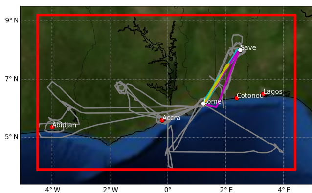
Figure 1. Map of the modeling domain (red rectangles) with location of the major cities (red dots), of the Lomé airport, and of the Savè super-site (white dots). Superimposed are the flight tracks of the three research aircraft during the 1–7 July 2016 period (gray lines). The aircraft flight tracks on 5 July are colored for the German Falcon (blue line), the French ATR 42 (violet line), and the British Twin Otter (yellow line).
