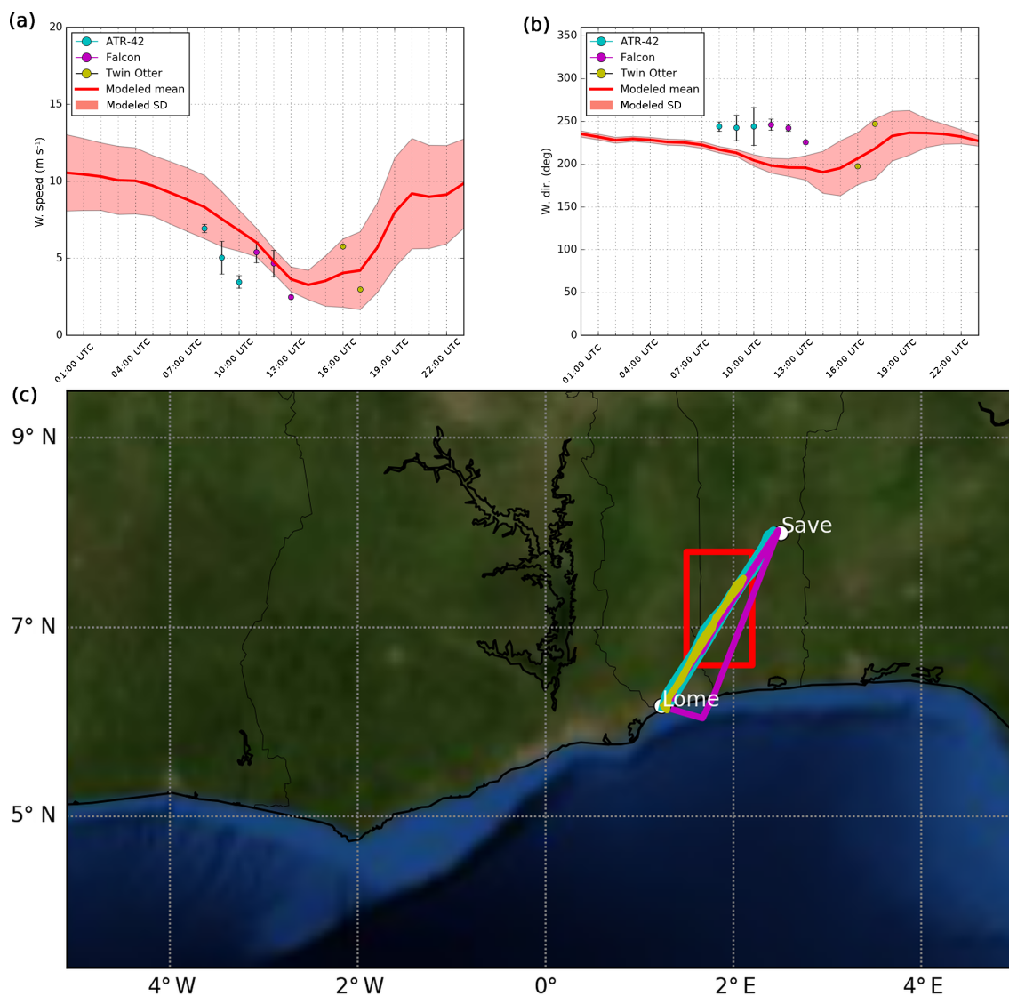
Figure A3. Wind speed (a) and direction (b) hourly averages and standard deviations on 5 July 2016 for all aircraft measurements (dots and error bars) acquired in a box (latitude from 6.6 to 7.8° N, longitude from 1.5 to 2.2° E, at an altitude from 300 to 1000 m). The horizontal extent of the box and the aircraft tracks are displayed on the map (c). Modeled value averages of the whole box are presented by the red line (and standard deviation by red shading). Blue dots correspond to ATR 42 measurements, violet to Falcon, and yellow to Twin Otter.
