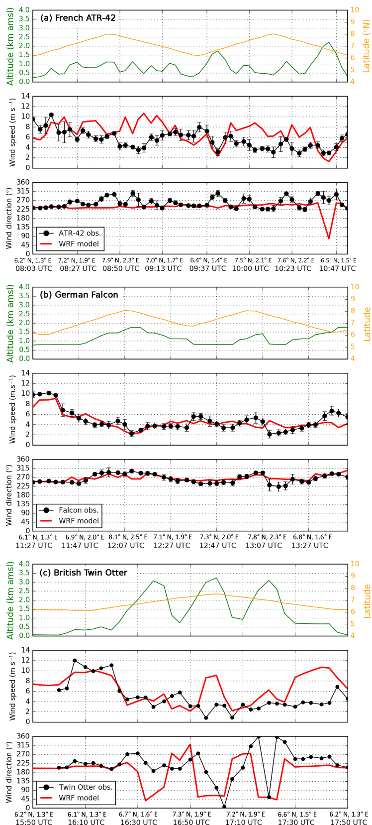
Figure 4. Time series on 5 July 2016 of (a) the French ATR 42, (b) German Falcon, and (c) British Twin Otter aircraft data, composed of three panels for each aircraft: (top) altitude (m) with the latitude (°N), (middle) wind speed (m s -1 ), and (bottom) wind direction (degrees). Modeled values with the WRF model are interpolated along the flight positions (red line). Observed value averages are the black dots with the hourly standard deviation (error bars).
