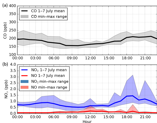
Figure 6. Hourly diurnal cycles of (a) carbon monoxide (CO in black), (b) nitrogen dioxide (NO 2 in blue), and nitrogen monoxide (NO in red) concentrations (ppb) observed at Savè (Benin). Means of each hour are presented by the lines over the period of 1–7 July 2016 and the upper and lower shading limits correspond to the hourly ranges (maximum and minimum of each hour over the period).
