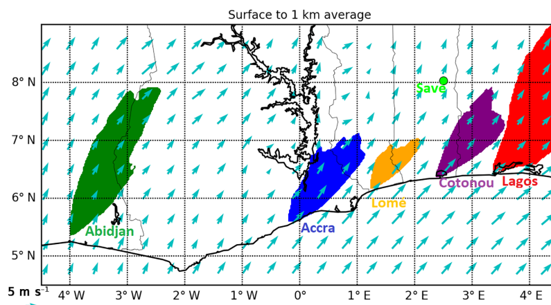
Figure 7. Maps of URB tracer concentration (in arbitrary units) averaged over the period of 1 to 7 July 2016 in the monsoon layer (from the surface to 1 km a.m.s.l.). Tracers are released from Abidjan (Côte d'Ivoire) in green, from Accra (Ghana) in blue, from Lomé (Togo) in orange, from Cotonou (Benin) in violet, and from Lagos (Nigeria) in red. The same threshold of tracer concentration is used for all city plumes for the color shading (Iso1). Wind vectors at 10 m modeled by WRF are presented by the light blue arrows. The location of the DACCWA super-site (Savè in Benin) is presented by the light green dot.
