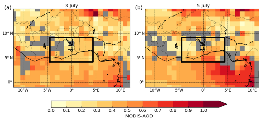
Figure 2. MODIS AOD 1-day moving average of two products acquired by Aqua and Terra (the combined Dark Target and Deep Blue MYD08-D3 and MOD08-D3 products, respectively) on 3 July 2016 (a) and 5 July 2016 (b). Data excluded by the cloud screening process are in gray. The modeling domain is presented by the black square.
