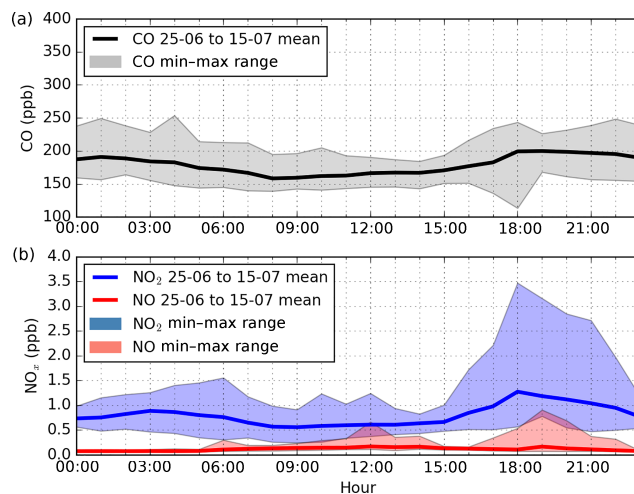
Figure A5. Hourly diurnal cycles of (a) carbon monoxide (CO in black), (b) nitrogen dioxide (NO 2 in blue), and nitrogen monoxide (NO in red) concentrations (ppb) observed at Savè (Benin). Means of each hour are presented by the lines over the entire campaign period (25 June to 15 July 2016). The upper and lower shading limits correspond to the hourly ranges (maximum and minimum of each hour over the period).
