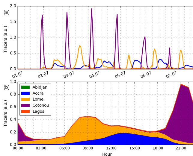
Figure 8. Time series of hourly URB tracer concentrations (in arbitrary units) modeled by the CHIMERE model at the DACCWA field campaign ground station in Savè (Benin) for the period of 1–7 July 2016. Urban tracers are released from five coastal cities: Abidjan (Côte d'Ivoire) in green, Accra (Ghana) in blue, Lomé (Togo) in orange, Cotonou (Benin) in violet, and Lagos (Nigeria) in red.
