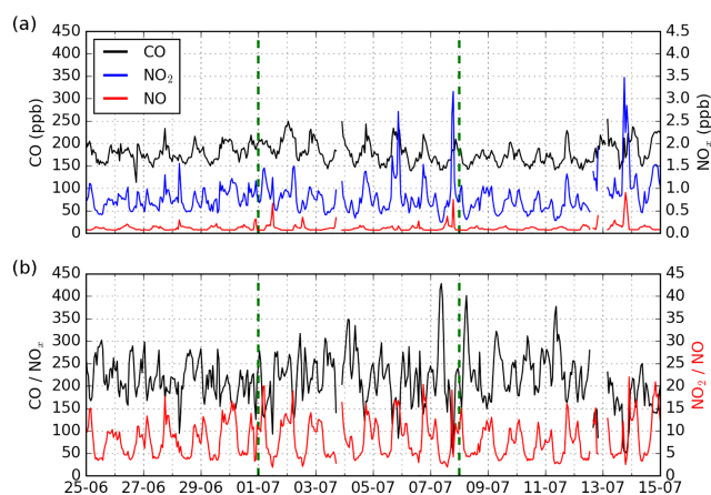
Figure A4. Time series of (a) carbon monoxide (CO), nitrogen dioxide (NO 2 ), and nitrogen monoxide (NO) hourly concentrations (ppb) observed at Savè (Benin) over the entire campaign period (25 June to 15 July 2016) and (b) of the ratios CO/NO x (in black) and NO 2 /NO (in red). The studied period (1–7 July 2016) is defined by the two green dashed vertical lines.
