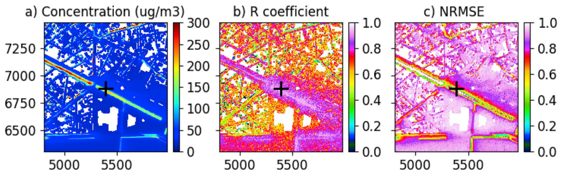
Fig. 4. Champs-Élysées Avenue area NO_x concentration (a), NO_x correlation coefficient (b), NO_x NRMSE on the 2nd of March 2016.
