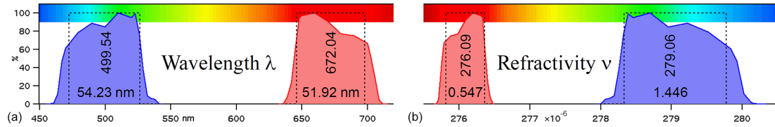
Figure 3. (a) GOMOS optical filter response as a function of wavelength. (b) Refractivity bandwidth of the GOMOS optical filters.
