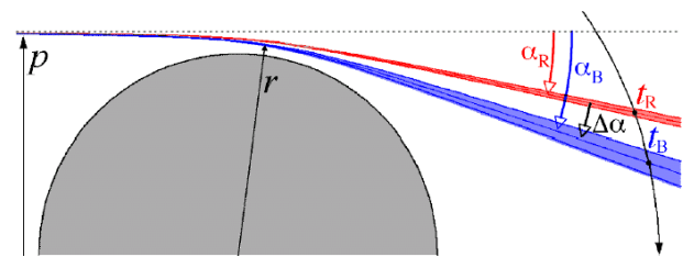
Figure 2. A scheme of chromatic refraction and the principle of refraction angle measurement by GOMOS. Both the refraction angles and the effect of dispersion are strongly exaggerated. However, the width of each beam relative to the angle difference \Delta\alpha is realistic. The impact parameter p is the geometric distance of the ray from the Earth's center. The vertical separation of blue and red rays at the ray perigee of 30 km is \sim 10 m (Dalaudier et al., 2001).
