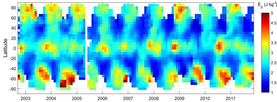
Figure 12. Time series of GW potential energy (zonal average) estimated from GOMOS HRTPs in the years 2002–2011.
