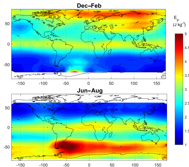
Figure 11. GW potential energy in two seasons, in the years 2002–2011.
