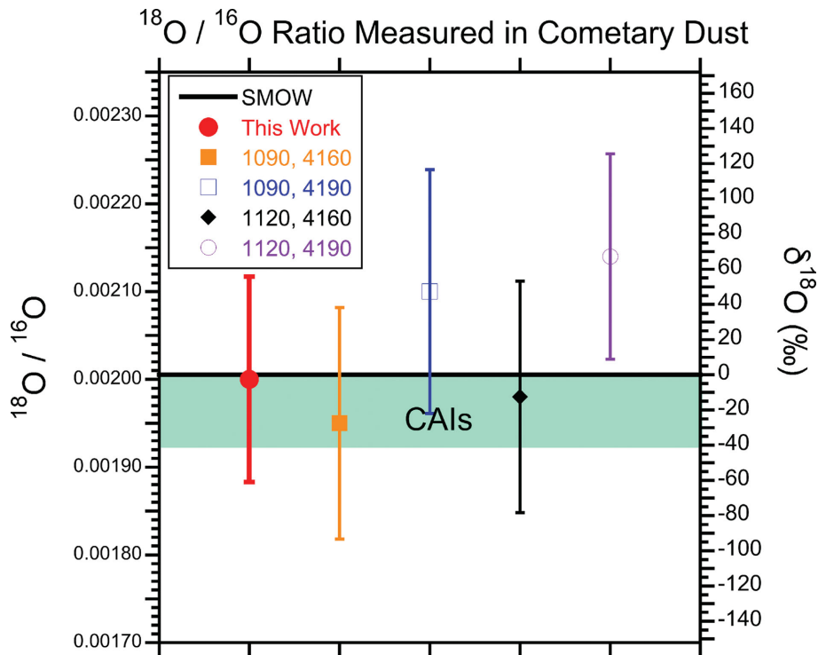
Figure 8. Comparison of the oxygen isotopic ratio from the long measurement on Jessica Lummene.2 with the ratios from the four locations that comprised it, with VSMOW and a range typical of CAIs shown for reference. The locations are labeled by the relevant X and Y target coordinates in microns. The error bars of the ratios from individual locations are necessarily larger from simple statistical considerations. While the two ratios at Y = 4160 are somewhat lower than VSMOW, they agree with it within errors. The two ratios at Y = 4190 are somewhat higher than VSMOW.
