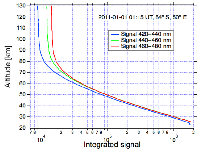
Figure 1. Spectrometer signal integrated in the three 20 nm spectral ranges for one occultation on 1 January 2011 (star ID = 3, orbit number = 46 209), lower background spectrum.
