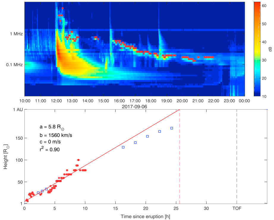
Figure 2. (top) Dynamical spectra of the radio emission following CME 3 from 6 September, selected data points (red asterisks), and (bottom) the resulting propagation profile and fit. The fit is compared with distance-time data points from Solar Terrestrial Relations Observatory (STEREO-A)/Sun-Earth Connection Coronal and Heliospheric Investigation (SECCHI)/Heliospheric Imager (HI) white-light shock observations (blue squares), which have been derived from J-maps. The dashed red line in the bottom panel marks the estimated time of arrival from the fit, while the black line marks the true time of arrival (TOF) of IP shock 2.
