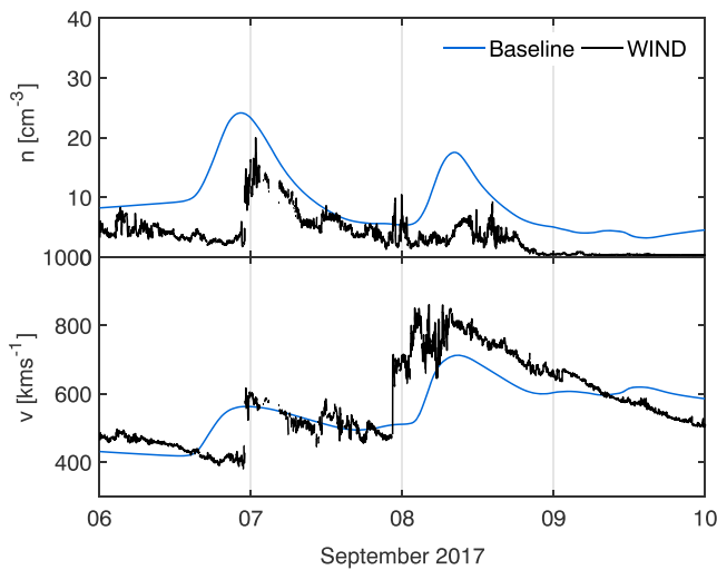
Figure 4. Output at L1 from the WSA-ENLIL+Cone baseline run and WIND data.
