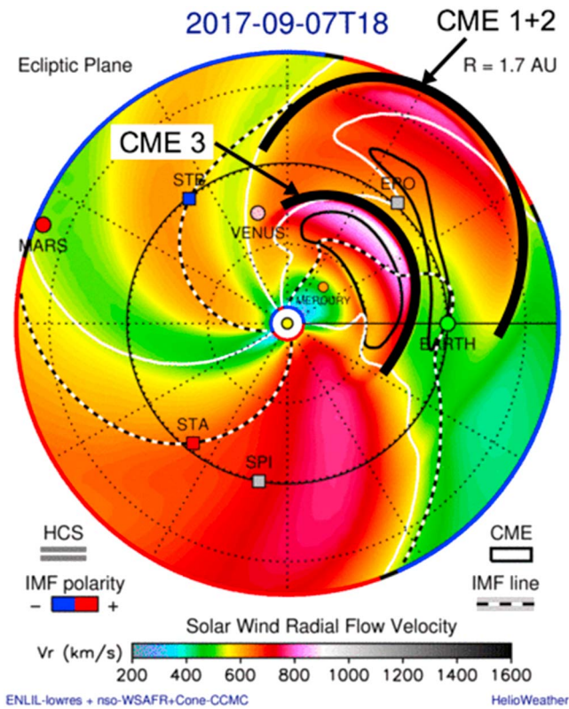
Figure 5. The radial solar wind velocity output from the baseline run as shown in the ecliptic plane. This snapshot from 7 September 18:00 UTC illustrates the longitudinal extent of all three coronal mass ejections (CMEs). See also Figure 4 for the output at L1. The full video is available in the HTML version of this paper or in the supporting information S1.
