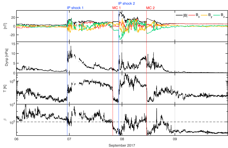
Figure 1. The 1-min averaged magnetic field and plasma data as detected by WIND at L1. The first panel (top to bottom) displays all magnetic field components in the geocentric solar magnetospheric system and |B| . The second panel shows the dynamical pressure, the third the proton temperature, and the fourth panel displays the plasma \beta ratio. The dashed horizontal line in panel 4 marks the \beta = 1 line, which enables the identification of dominant magnetic structures (i.e., magnetic clouds; MCs). The dotted vertical lines across all panels signifies the arrival of interplanetary (IP) shocks 1 and 2 (blue), while the vertical lines in red represent the arrivals of MCs 1 and 2.
