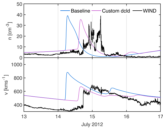
Figure 8. Baseline and custom dclD output from the WSA-ENLIL+Cone model and WIND data for the 12 July 2012 coronal mass ejection event.
