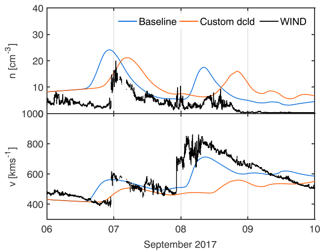
Figure 7. Output from the WSA-ENLIL+Cone model custom run compared to the baseline run and WIND data.
