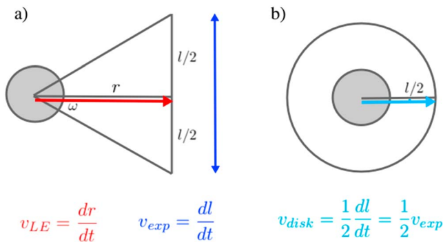
Figure 3. Schematic showing the line-of-sight view for a cone coronal mass ejection erupting on the limb (a) and a halo coronal mass ejection (b). Figure adapted from Gopalswamy et al. (2009).
