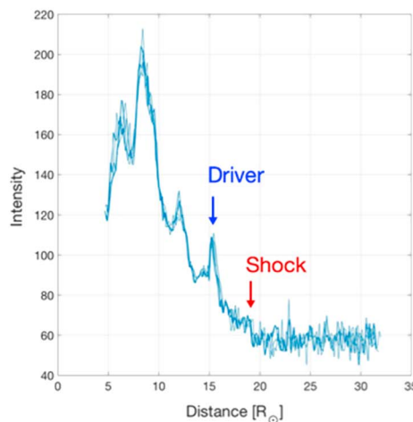
Figure 6. The dcl cuts (left) taken along the dashed white line (right). The input to WSA-ENLIL+Cone has been taken as the ratio between the intensity of the shock front, as marked by the red arrow (left) and the ambient solar wind. The blue arrow (left) and the dashed blue curve (right) marks the CME driving the shock (“Driver”).
