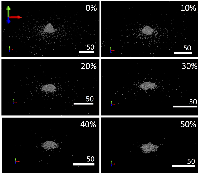
Fig. 6. 3D view of a RLPA aggregate after projection with different mass loss. A scale is given in number of monomers, and a referential frame is indicated by colored arrows (x = blue, y = red, and z = green) with an approximate 30° viewing angle.
