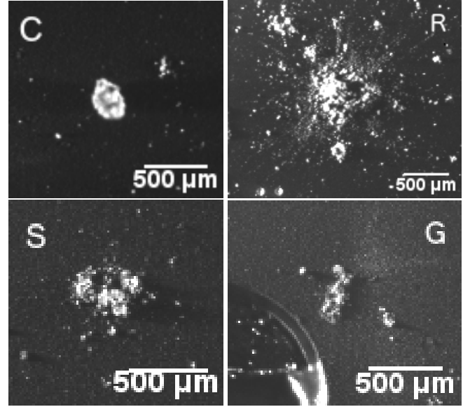
Fig. 1. Diversity of crushed particle types detected by COSIMA (Nick: compact particle, C; Alexandros: rubble pile, R; Estelle: shattered cluster, S; and Johannes: glued cluster, G; adapted from Langevin et al. 2016 ).
