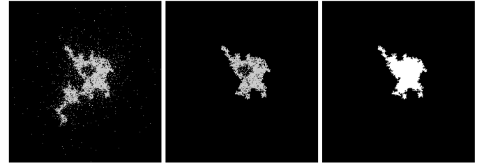
Fig. 7. Illustration of the connected area calculated for a flattened aggregate of type RLCA. The flattened particles seen from above is shown on the left. The calculated connected areas are shown with gaps in the middle and without gaps on the right. The parts of the aggregate that are not connected to the largest connected aggregate are removed from the processing.
