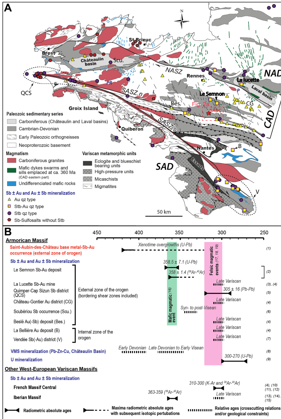
Fig. 1. A. Geological map of the Armorican Massif with location of the different Sb-Au mineralization types. The eastern parts of both the Central Armorican Domain (CAD) and the Cadomian northern domain suffered important basic magmatism attested by numerous dolerite dyke swarms and sills (in green) at ca. 360 Ma (Pochon et al. , 2016b). A high-density network of kilometre-scale NNW-SSE-trending vertical faults affects the CAD to the south of Rennes city. NASZ: North Armorican Shear Zone; SASZ.n.,s: South Armorican Shear Zone, northern and southern branches respectively; Champpt: Champptoceaux metamorphic complex; PR, L, P: Pontivy-Rostrenen, Lizio and Le Pertre granites respectively; SADC: Saint-Aubin-Des-Châteaux (red star). B. Age compilation of Sb-Au mineralized systems through the Western European Variscan orogenic segments. Armorican Base metal VMS and U mineralization have also been reported. The deposits or districts are localized on 1A (name abbreviation). (1) Tartèse et al. (2015), (2) Pochon et al. (2018), (3) Chauris and Marcoux (1994), (4) Bouchot et al. (1997), (5) Marcoux and Fouquet (1980), (6) Pierrot et al. (1975), (7) Marcoux et al. (1984), (8) Lescuyer et al. (1997), (9) Ballouard et al. (2018a), (10) Charonnat (2000), (11) Bouchot et al. (2005), (12) Chauvet et al. (2012), (13) Couto et al. (1990), (14) Neiva et al. (2008), (15) Hall et al. (1997), (16) Pochon et al. (2016b), (17) Augier et al. (2015), (18) Capdevila (2010), (19) Ballouard et al. (2018b).
