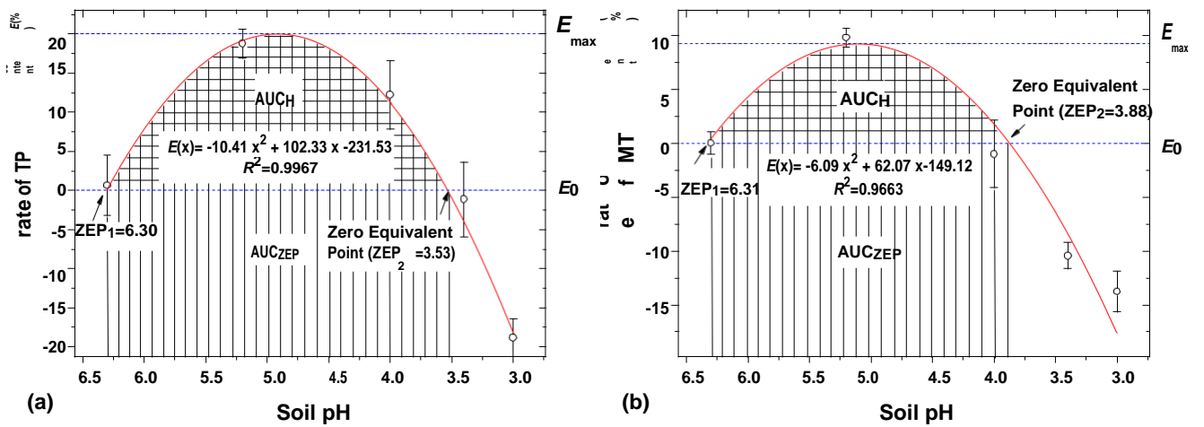
Fig. 2 Total protein (TP) and metallothionein (MT) contents in Eisenia fetida after 28 days of exposure to five soil pH levels (n = 3). E_0 is the zero effect; E_{max} is the maximal stimulatory effect; ZEP_i (i = 1, 2) is the zero equivalent point; AUC_H is the area under the hormetic zone, and the
