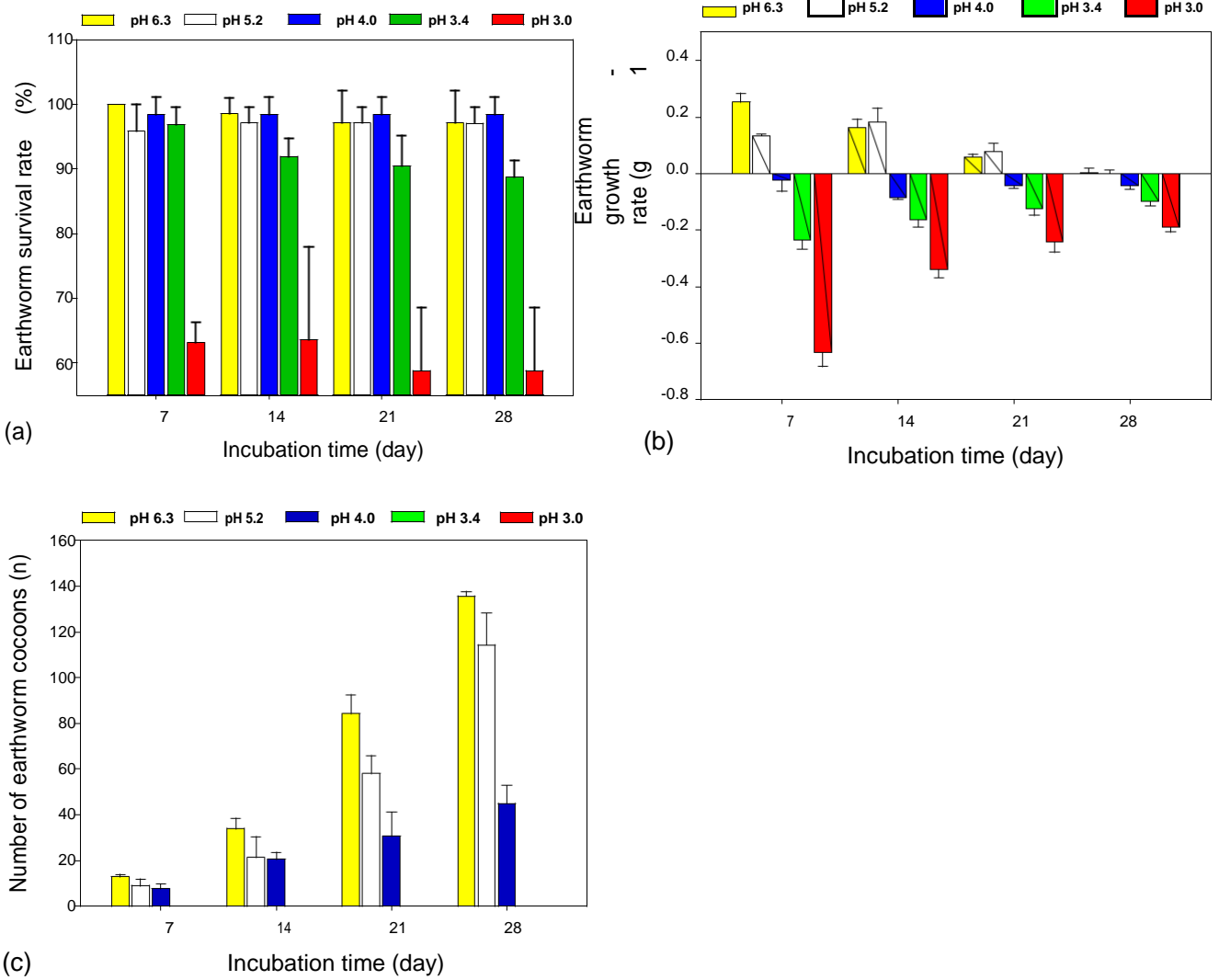
Fig. 1 Survival rate (a), growth rate (b), and cocoon production (c) of Eisenia fetida exposed to different soil pH levels (mean \pm standard deviation, n = 3)
