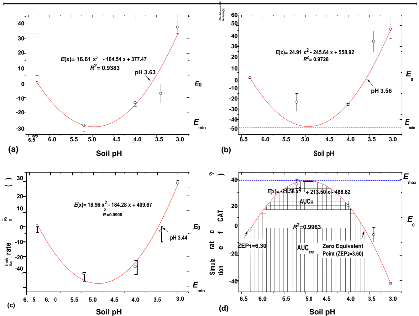
Fig. 3 The GSH-PX, SOD, POD, and CAT activities in Eisenia fetida after 28 days of exposure to five soil pH levels ( n = 3 ). E_0 is the zero effect; E_{max} and E_{min} are maximal stimulatory effect and minimum stimulatory effect, respectively; ZEP_i ( i = 1, 2 ) is the zero equivalent
