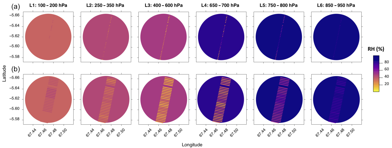
Figure 9. Example of predicted RH for a single SAPHIR pixel corresponding to ice cloud profiles using, within the iterative scheme, the QRF method (a, median) and the geoaddivitive model (b). The disks correspond to the SAPHIR footprints and the dots inside to the RH predictions at CALIPSO resolution. Although CALIOP accumulates data over 330 m along track, here for figure clarity we assumed the profiles to be symmetric and doubled their radius.
