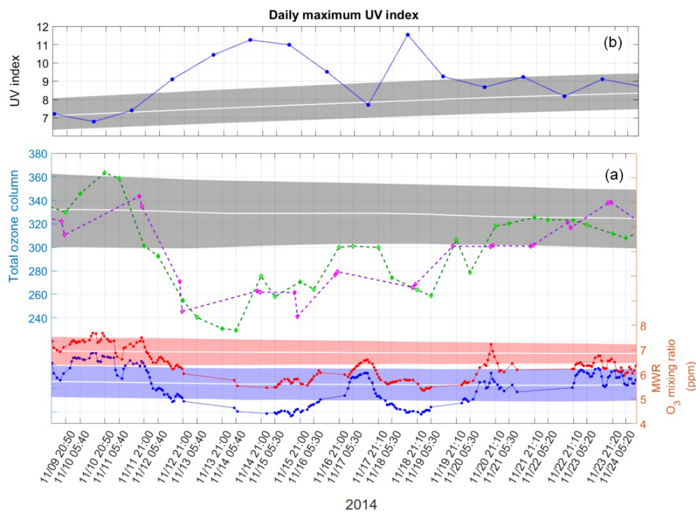
Figure 7. Atypical event of Antarctic ozone hole influence over Río Gallegos. (a) Time evolution of the MWR ozone mixing ratio at 27 km (blue line) and 37 km (red line). Light red and light blue areas represent the ozone mixing ratio zonal climatology at both altitudes calculated using the MLS database (2004–2016). (a) Time evolution of the total ozone column measured with the ground-based SAOZ instruments (green dots) and OMI (purple dots) in Dobson units. White line and grey area represent the climatology and 1 SD calculated using the OMI database (2004–2017). (b) Time evolution of the daily maximum Ultraviolet Index measured with the YES UVB-I ground-based solar radiometer at the OAPA. White line and grey area represent the climatological UVI at noon in Río Gallegos.
