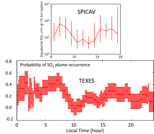
Fig. 19. Top panel: SO 2 volume mixing ratio, as observed by SPICAV aboard Venus Express at an altitude of 70 km as a function of local time, including all data between 2006 and 2015. Bottom panel: probability of occurrence of an SO 2 plume as a function of local time, including TEXES data between 2012 and 2018 (see Fig. 11).
