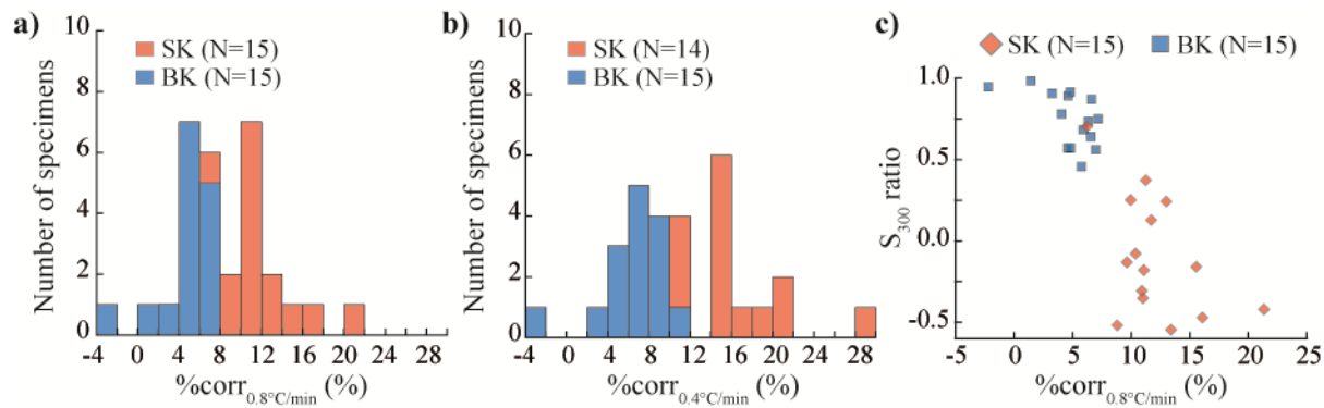
Figure 5: Histograms of cooling rate correction factor %corr for 0.8°C/min (a) and 0.4°C/min (b), cooling rates from 650°C for SK bricks and from 555°C for BK bricks; (c) S_{300} ratio versus cooling rate correction factors (0.8°C/min slow cooling).
