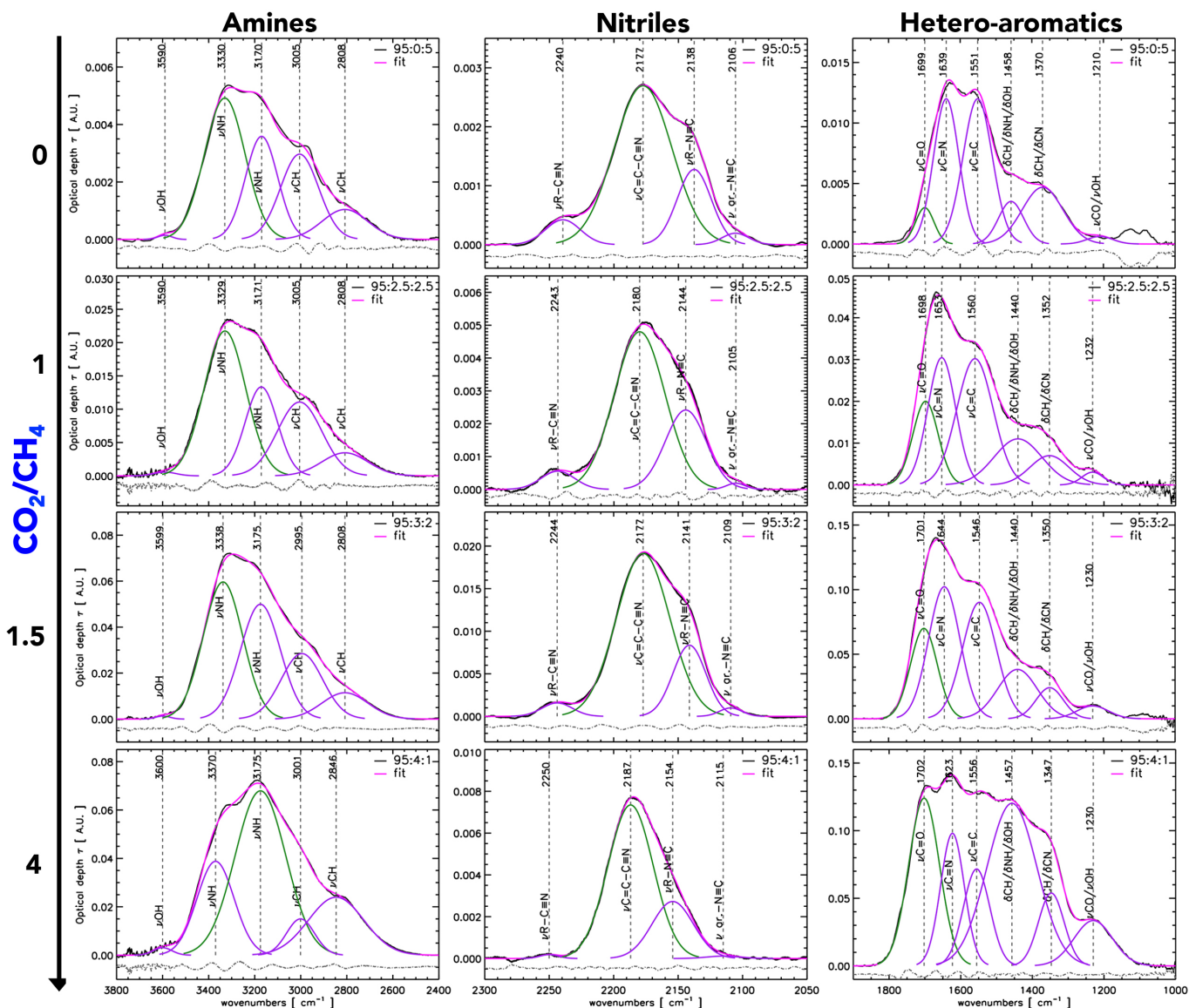
Figure 4. Spectral deconvolution of the main mid-infrared spectral bands (amines, nitriles, hetero-aromatics spanning 3800–1000 \text{cm}^{-1} ) of increasingly oxidized organic tholins. To illustrate the effect of the increasing \text{CO}_2/\text{CH}_4 ratio on the molecular structure, only tholins from the same series (95 % \text{N}_2 ) and varying \text{CO}_2/\text{CH}_4 ratios = 0, 1, 1.5 and 4, are used.
