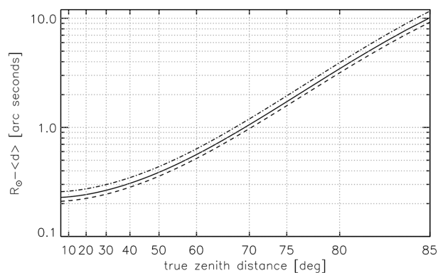
Figure 4. Difference between the true solar radius and the mean observed one as a function of the true zenith distance. The full line corresponds to average weather conditions at Calern ( T = 15^\circ\text{C} and P = 875 \text{ hPa} ). The dot-dashed and dashed lines correspond, respectively, to T = -10^\circ\text{C} , P = 900 \text{ hPa} and T = 30^\circ\text{C} , P = 850 \text{ hPa} . All calculations are made using the exact formulae equations (18) and (46) for Calern station assuming 50 per cent humidity.
