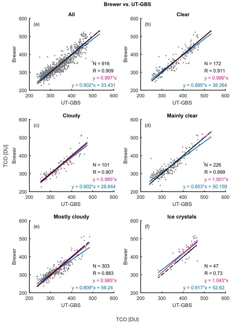
Figure 6. Scatter plots of Brewer total column ozone vs. UT-GBS TCO. Panel (a) shows the scatter plot of all coincident measurements of Brewer and UT-GBS. Panels (b) to (f) show scatter plots with weather conditions indicated in their titles. On each scatter plot, the red line is the linear fit with intercept set to 0, the blue line is a simple linear fit, and the black line is the one-to-one line.
