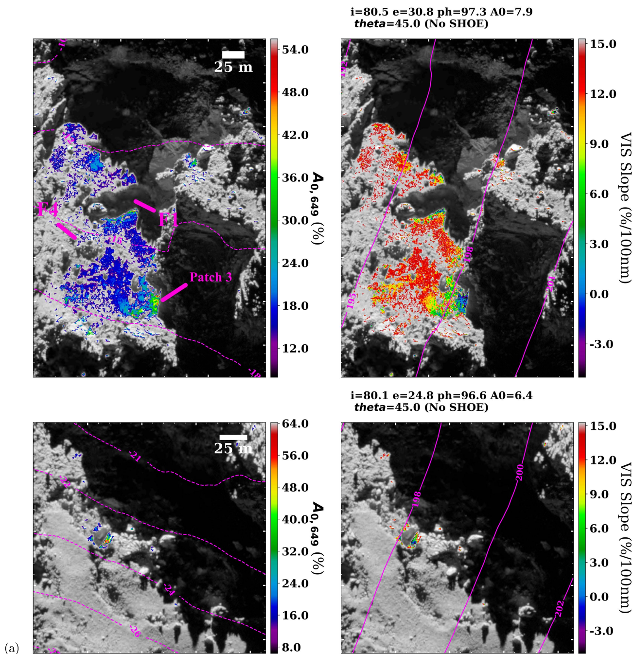
Fig. 6. NAC F22 normal albedo and VIS spectral slope of Khonsu bank before and after perihelion passage. Normal albedo and VIS slope are overplotted on their RGB composites. (a) January 16, 2015, UTC 01:27 divided into two panels that show the High and Low banks. The median VIS spectral slope is 15.95%/100 nm.
