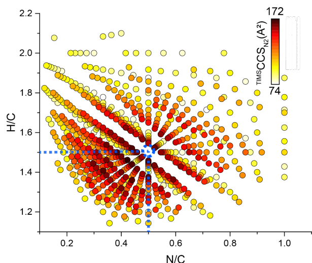
Figure 2. H/C versus N/C van Krevelen representation of all C_xH_yN_z -class constituents color-coded according to peak apex TIMS CCS_{N_2} -value. A clear center of the pattern can be seen at H/C 1.5 and N/C 0.5 (marked in blue).
