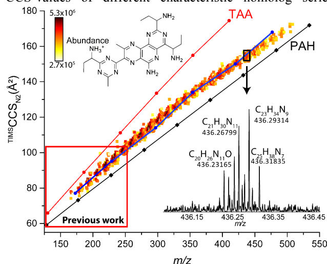
Figure 1. Apex collision-cross-section ( ^{TIMS}CCS_{N_2} , at room temperature) versus m/z color-coded by abundance. The behavior of the theoretical cross-sections of different structural motif is provided for tetraalkylammonium salt species (TAA, red) and polycyclic aromatic hydrocarbons (PAH - black). A proposed structural motive for the tholins homolog series is presented in blue (archipelago ramified N-PAH). The mass spectrometric excerpt of the nominal mass 436 visualizing the high isobaric complexity. Detailed information on the homolog rows can be found in Table S1 and Figure S1.
