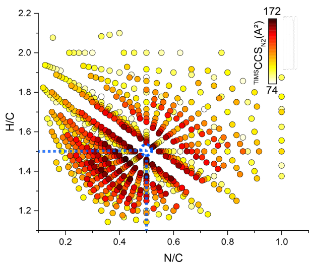
Figure 2. H/C versus N/C van Krevelen representation of all C_xH_yN_z -class constituents color-coded according to peak apex TIMS^MS CCS_{N_2} -value. A clear center of the pattern can be seen at H/C 1.5 and N/C 0.5 (marked in blue).
