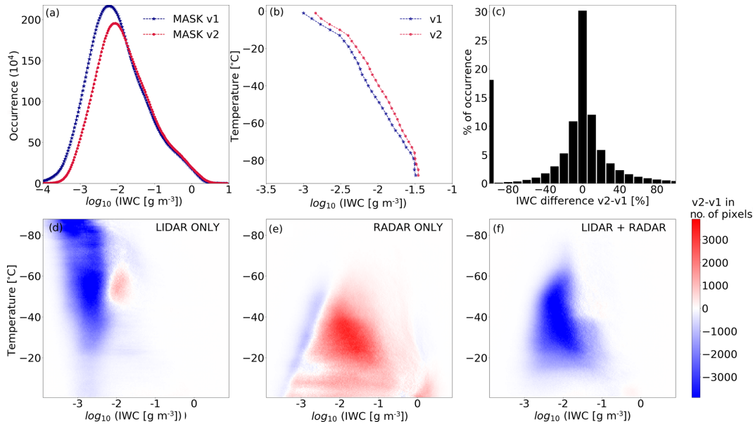
Figure 5. Comparison of DARDAR-MASK v1 and DARDAR-MASK v2 in terms of IWC retrieved using Varcloud ( V_2 ): histograms of \log_{10}(\text{IWC}) (a) with the old version of DARDAR-MASK in dashed line and the new version in solid line, the mean of the distribution of \log_{10}(\text{IWC}) as a function of temperature (b) for DARDAR-MASK v1.1.4 (dashed line) and DARDAR-MASK v2.1 (solid line), the histogram of the relative difference \frac{\text{IWC}_{v2} - \text{IWC}_{v1}}{\text{IWC}_{v1}} between DARDAR-MASK v2 and DARDAR-MASK v1 (c), and the difference between the two configurations in terms of number of pixels in each [T - \log_{10}(\text{IWC})] bin for lidar-only pixels (d), radar-only pixels (e), and pixels combining the two instruments (f).
