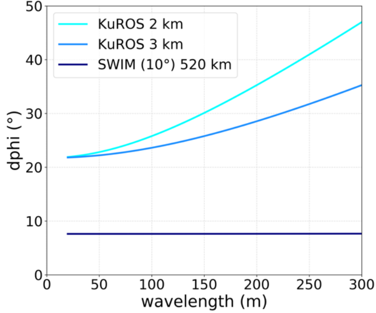
Figure 2. Directional selectivity for the two KuROS altitudes and for the 10° incidence beam of the SWIM instrument onboard the CFOSAT mission.
