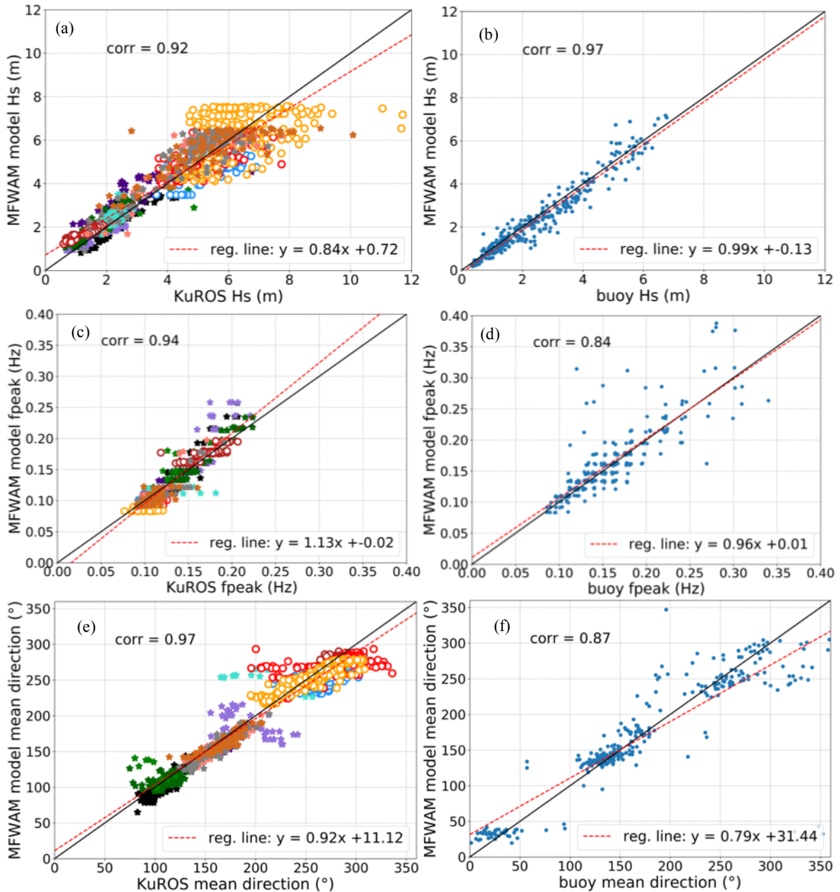
Figure 11. Overall comparisons of the MFWAM-run2 principle wave parameters ( H_s , f_{\text{peak}} and \phi_{\text{mean}} ) during the HyMeX campaign with the KuROS (left-hand side) and the Tri-axis buoy (right-hand side) data. In Figures (a), (b) and (c) there are 1271 measurement points. Each color represents one flight. Star symbols are for flights in fetch-limited conditions, open circles are for flights in easterly high wind conditions. For remainder, buoy data are analyzed over 1 month between the 5 th of February and the 15 th of March 2013. For the buoy comparison, there are 307 measurement points.
