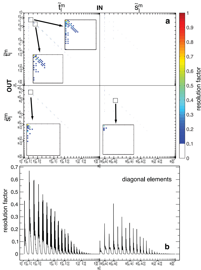
Figure A1. Model resolution matrix \mathbf{K}_R \mathbf{M} for the 2001 near-surface flow inversion of Fig. 12 (using prior model 3). (a) Full matrix, (b) diagonal coefficients.
