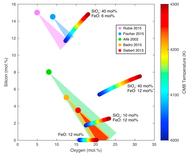
Figure 3. Results of thermodynamic modeling showing core compositions in equilibrium with a pyrolytic lower mantle, a lower mantle enriched in ferropericlase and depleted in \text{SiO}_2 , and two intermediate compositions (thick colored lines, with colored gradient scale on the right indicating CMB temperature). Compositions at higher and lower temperatures can be inferred by extrapolation. Solid colored circles correspond to core compositions found in the literature [Rubie et al. , 2015, Fischer et al. , 2015, Alfe et al. , 2002, Badro et al. , 2015, Siebert et al. , 2013]. The fans leading from those compositions come from Figure 2 and show changes to the Si and O content which would result in a slower and lighter layer. If the core contains a relatively high concentration of Si (i.e., Rubie et al. [2015] or Fischer et al. [2015]), then a reaction between a cool core ( T < 4000 K) and a pyrolytic mantle can produce a light and slow layer, as shown by the fans spreading from those compositions. Core compositions with less silicon [i.e., Badro et al. , 2014; Alfe et al. , 2002; Siebert et al. , 2013] cannot produce an E' layer from a reaction with a pyrolytic mantle. However, these compositions can evolve toward a light and slow layer if they react with an FeO-enriched lower mantle.
