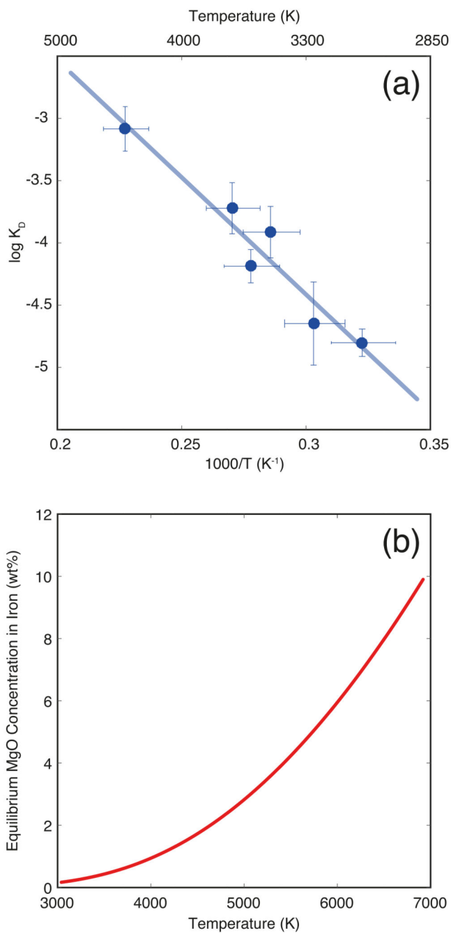
Figure 1. Magnesium solubility in metallic iron melt at high pressure and temperature. (a) Equilibrium constant for MgO dissolution in iron as a function of reciprocal temperature (Eq. 2). The experimental data is from Extended Data Table 1. The line corresponds to the least-squares linear fit to the data. A comparison with extrapolation from DFT calculations 4 is shown in Extended Data Fig. 2. (b) The resulting MgO concentration in iron in equilibrium with pyrolite as a function of temperature. This is obtained by rewriting (Eq. 2) to obtain X_{Mg}^{metal} = 2.91 \cdot \exp\left(-\frac{21662}{T}\right) , where T is temperature in K, and then converting
