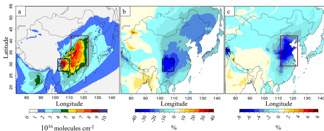
Figure 8. (a) Ammonium columns (molecules \text{cm}^{-2} ) for the 2015A simulation, (b) relative differences of ammonium columns between the simulations from 2015B and 2015A, in %, and (c) additional relative differences of ammonium columns between the simulations from 2015C minus 2015B compared to 2015A, in %. The black rectangle is for the Sichuan Province and Chongqing municipality, and the red rectangle is for northern China.
