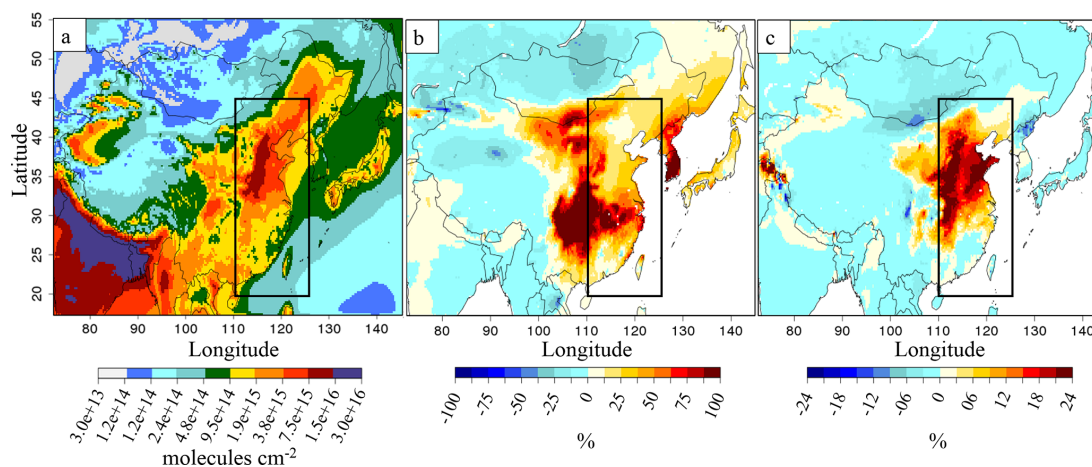
Figure 7. (a) Ammonia columns (molecules \text{cm}^{-2} ) for the 2015A simulation, (b) relative differences of ammonia columns between the simulations from 2015B and 2015A, in %, and (c) additional relative differences of ammonia columns between the simulations from 2015C minus 2015B compared to 2015A, in %. The black rectangle is for the eastern China domain.
