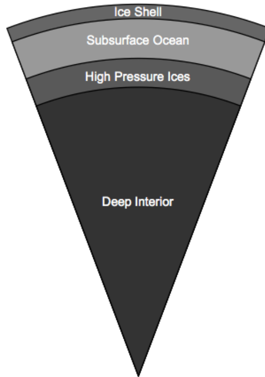
Figure 4. Probable present-day structure of Titan's interior showing that Titan is internally differentiated, with a deep rocky or rock-ice mix deep interior.
