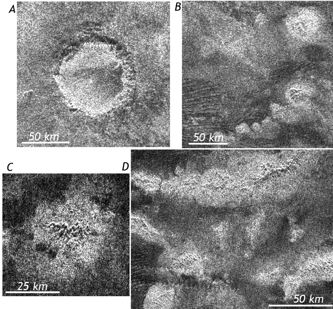
Figure 11. Some examples of mountains on Titan. Radar illumination is from the top in all cases, and north is up. Bright, possibly erosional, blankets surround the central, high elevation features visible as bright/dark pairs. (a). Sinlap Crater, shown to demonstrate the effects of radar illumination on a rimmed depression. (b). Individual mountain blocks in the T3 swath south of Sinlap crater. (c). Rugged mountain from the T3 swath. (d). A portion of mountain ranges west of the Huygens landing site from the T8 swath. From Radebaugh et al. (2007).
