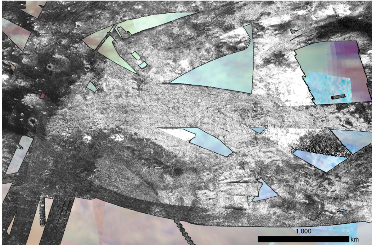
Figure 16. Xanadu region. All Cassini SAR and HiSAR image swaths covering the Xanadu region, overlain on a VIMS basemap. Xanadu is generally SAR-bright because of rough terrain and fractured ice, which is interspersed with valleys filled with SAR-darker sediment. Some regions of Xanadu are VIMS dark blue, consistent with the presence of exposed water ice. The southwest margin of Xanadu has large river channels emptying to the south.
