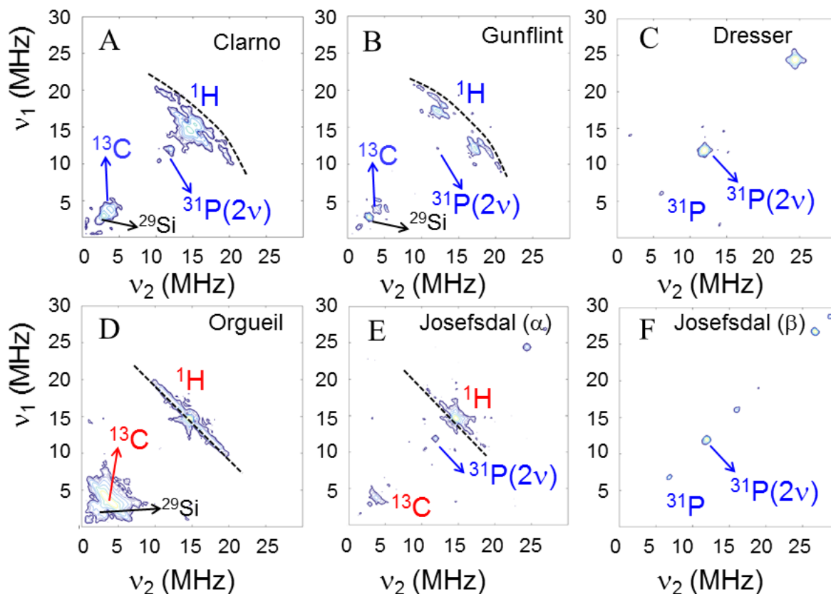
Fig.7. HYSORE spectra at 5 K of A) a chert from the Clarno Formation, John Day Basin Tectonic Unit, Oregon, USA (0.045 Ga); B) a chert from the Gunflint Formation, Schreiber Beach locality, Ontario, Canada (1.88 Ga); C) a chert from the Dresser Formation, Warrawoona Group, Pilbara craton, Australia (3.48 Ga); D) IOM of the Orgueil meteorite; E) and F) samples \alpha and \beta , respectively, of the Josefsdal Chert, Barberton Greenstone Belt, South Africa. The dotted lines in A, B, D, E highlight the shape of the proton ridge in biogenic and meteoritic IOM. All 2D HYSORE spectra were recorded at a \tau value of 136 ns, with 256x256 points in both t_1 and t_2 dimensions.
