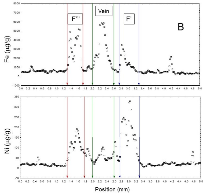
Fig.8. A) Optical image of horizon F with laminae F ''' and F ' . The chert vein crossing horizon F is highlighted by dashed lines. The black box represents the area scanned by the proton beam (5 mm x 0.5 mm) by steps of 20 µm (250 x 25 pixels). PIXE images of Fe, Ni and Cr are shown on the bottom. B) Projection on x-axis of data for Fe and Ni. Each compositional result was obtained from the fitting of the spectra grouped over the 25 vertical pixels for each horizontal position of the beam. Data corresponding to lamina F ' and F ''' and the vein are delineated by blue, red and green vertical lines, respectively.
