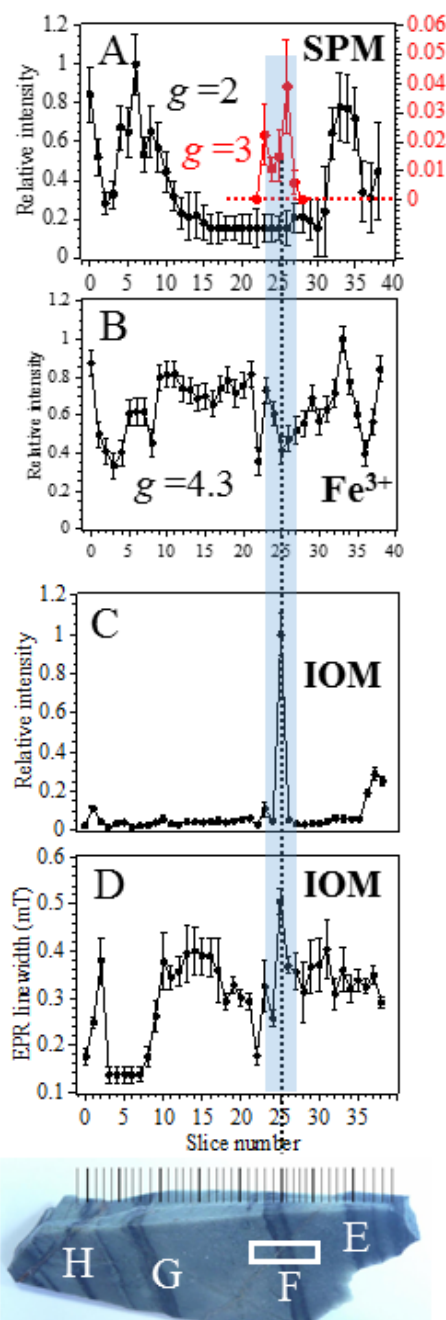
Fig.4. Variation of cw-EPR spectra in the 40 slices of sample \alpha shown at the bottom of the diagram (the location of this sample in the context of the outcrop is shown by a rectangle in Figure 1C). The slices, labelled 0 to 39 along the abscissa of (D), were collected parallel to the stratification. In terms of stratigraphy, slice 0 (to the left) corresponds to the stratigraphic top of the sample and slice 39 to the bottom (to the right). The image of sample \alpha is shown with the position of the 40 slices studied by EPR (vertical bars) and four black horizons (labelled E to H). The white box represents the area scanned in the PIXE analysis (see Section 4.4.1). Data for the black horizon F (slices 23 to 26) are highlighted with a blue rectangle covering panels A-D. Slice 25 comprises a large part of lamina F' of horizon F and is highlighted by a discontinuous vertical line. (A) EPR intensity profile of the superparamagnetic resonance signal (SPM) of possibly ferrite nanoparticles ( g = 2 ), and of the signal at g = 3 attributed to Ni-Cr-Al ferrite nanoparticles; (B) EPR intensity profile of \text{Fe}^{3+} impurities ( g =
