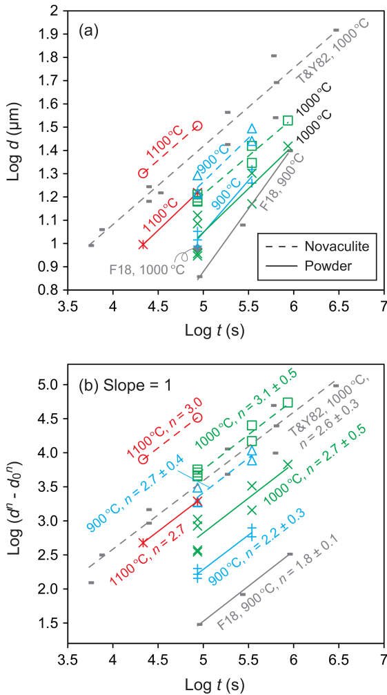
Figure 8. Grain sizes at a pressure of 1.5 GPa and for different durations; (a) log d ; (b) log ( d n - d 0 n ) with changing n values to obtain slopes = 1. Grain sizes in micrometers (μm). Also shown are data from Tullis and Yund (1982) (denoted as T&Y82) for novaculite and from Fukuda et al. (2018) (F18) for powder.
