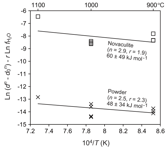
Figure 10. Dependence of temperature on grain size. Pressure of 1.5 GPa. Grain sizes in micrometers (μm) and water fugacity in megapascals (MPa).
