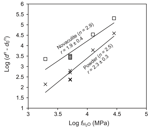
Figure 9. Dependence of water fugacity on grain size. Temperature of 1000 °C and pressures of 1.0, 1.5, 2.0, and 2.5 GPa. Grain sizes in micrometers (μm).
