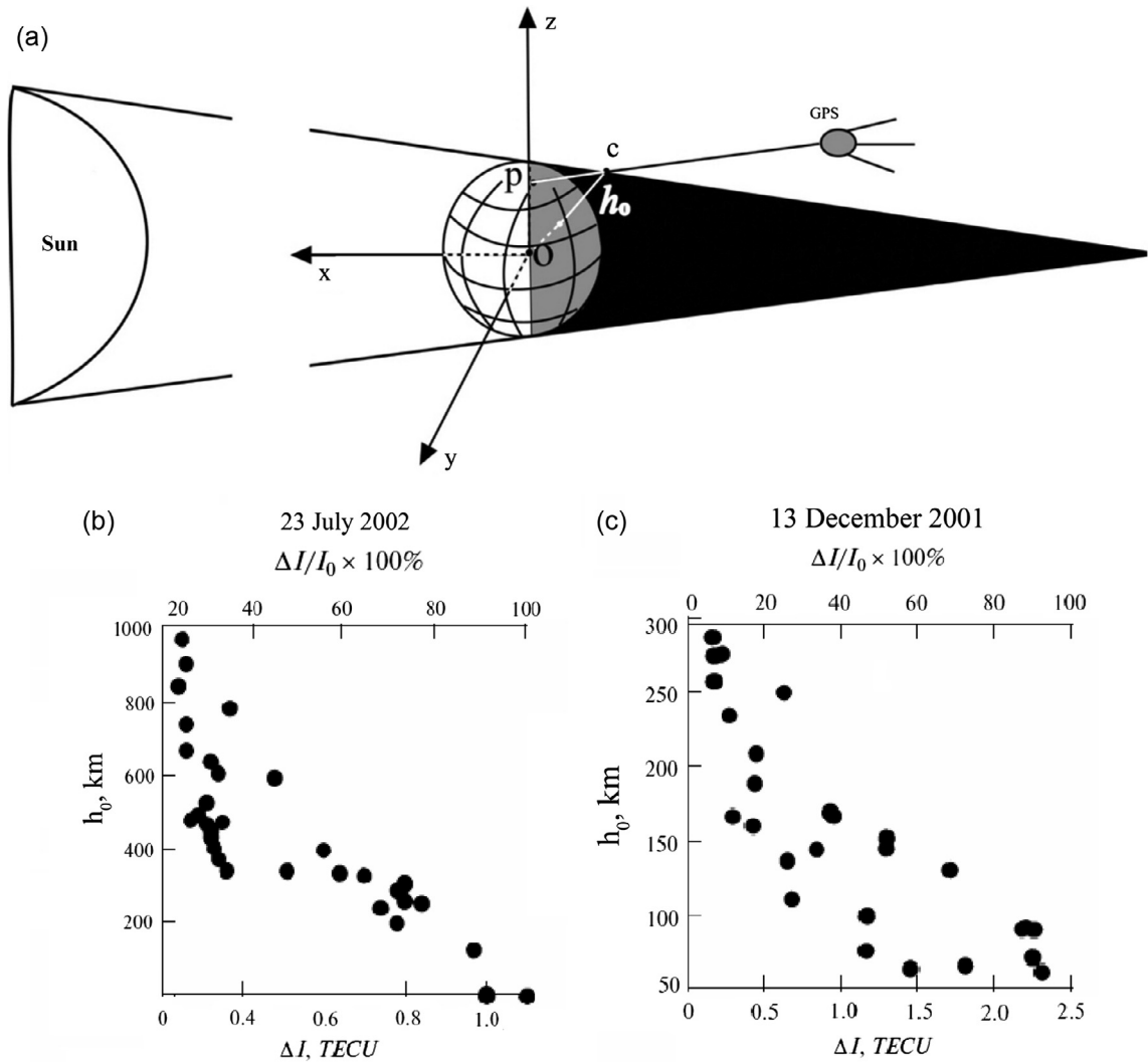
Fig. 5. (a) Pattern of the shadow of the Earth on its atmosphere (figure taken from Afraimovich & Perevalova 2006 ). (b, c) Two types of the TEC absolute increment \Delta I depending on the shadow height h_0 ( Leonovich & Tashilin 2008 ).
