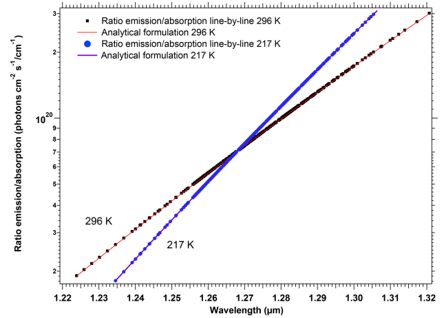
Figure A5. For two different temperatures (296 and 217 K), the ratios of our calculated emission rate to the HITRAN line strength SS are plotted (respectively, black and blue dots) for all 375 transitions of HITRAN table (between 1.2238 and 1.32068 μm). The solid lines (respectively, red and blue) are computed from the analytical formula (Eq. A13) on a grid of wavelength–wavenumber using the same scale on the left as the ratio of emission to line strength in units of photons \text{cm}^{-2} \text{s}^{-1} / \text{cm}^{-1} , where \text{cm}^{-1} is a wavenumber unit.
