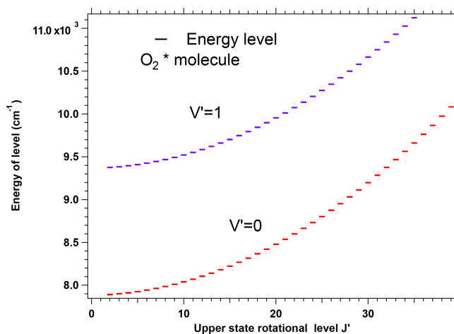
Figure A3. Energy levels (in \text{cm}^{-1} ) of the excited molecule O 2 * as a function of rotational and vibrational quantum numbers J' and V' .
