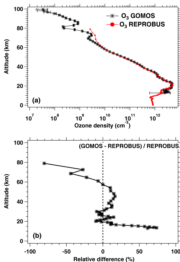
Figure C1. (a) One typical example of comparison of a GOMOS vertical ozone profile (black curve) versus REPROBUS prediction profile (red curve). The GOMOS profile was observed during the night on 8 January 2007. (b) Relative difference (\text{GOMOS} - \text{REPROBUS})/\text{REPROBUS} .
