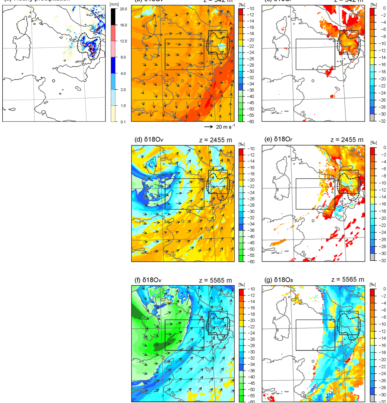
Figure 13. Same as Fig. 10 but for 00:00 UTC on 16 October 2012.
