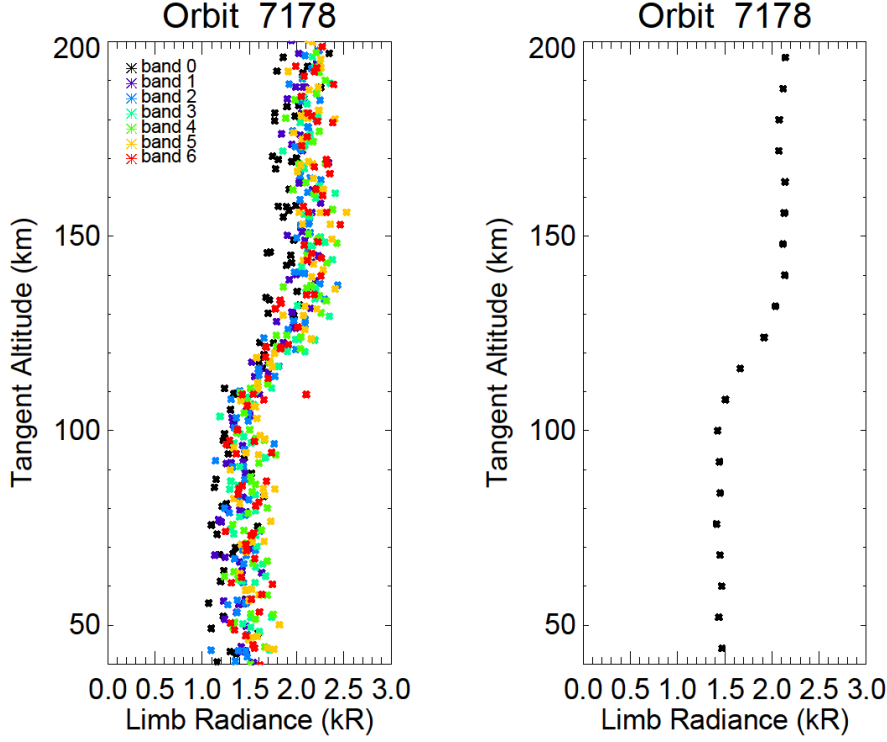
Figure. 2 : Left : Vertical profiles of the H Lyman- \alpha brightness measured at limb between 40 and 200 km for each of 7 spatial bins (labeled as “bands” and shown with different colors) during orbit 7178 for all six inbound limb scans, observed on 7 June 2018. The error bar for each individual value is \sim 0.13 kR. Right : Average profile derived with a vertical resolution of 8 km. The uncertainty on the mean is \sim 0.03 kR, lower than the thickness of the points.
