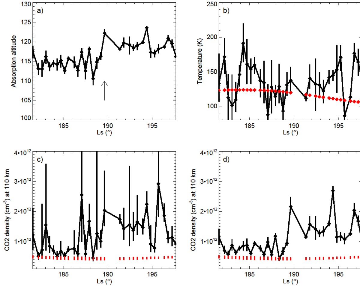
Fig. 4 a) Variations of the CO 2 absorption altitude (km), defined as the altitude where the slant CO 2 absorption optical thickness at Lyman- \alpha is equal to 1 with the solar longitude Ls. b) derived temperature for each orbit from the CO 2 scale height. c) variations of the CO 2 density with Ls considering the temperature derived from the fit. d) Same as c) but using a same temperature of 135 K for the full period. The range of temperature and CO 2 density at 110 km extracted from the Mars Climate Database at the same position are shown by red lines for panels 3b, 3c and 3d. The arrow on panel 3a indicate the time of orbit #7182.
