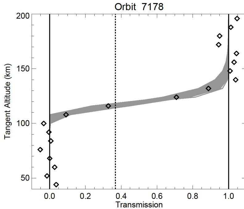
Fig. 3 Transmission function for orbit 7178 (diamonds) and the best fit derived using a function given by Eq. 3 (solid line). The two vertical solid lines indicate Transmission= 0 and Transmission =1. The vertical dotted line indicate Transmission = e^{-1} . Because I_0 and I_1 are average values between 40-80 km and 160-200 km respectively, the computed individual transmission values can be < 0 (when I(z) < I_0 ) near 100 km and > 1 (when I(z) > I_1 ) near 160 km respectively. The best fits obtained from a Monte Carlo error analysis are also displayed by the grey area.
