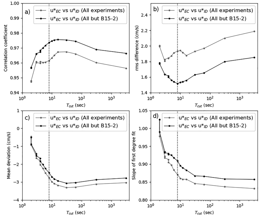
Figure 14. Sensitivity of the statistical elements of the comparisons between ID and EC u^* estimates as a function of the cutoff Period ( T_{cut} ) of a high-frequency pass filter applied to EC data.
