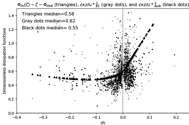
Figure 15. Comparison of the dimensionless dissipation function (triangles) to composite estimates of the dissipation rate that are either normalized with respect to u_{*EC}^3 (gray dots) or with respect to u_{*bulk}^3 (black dots).
