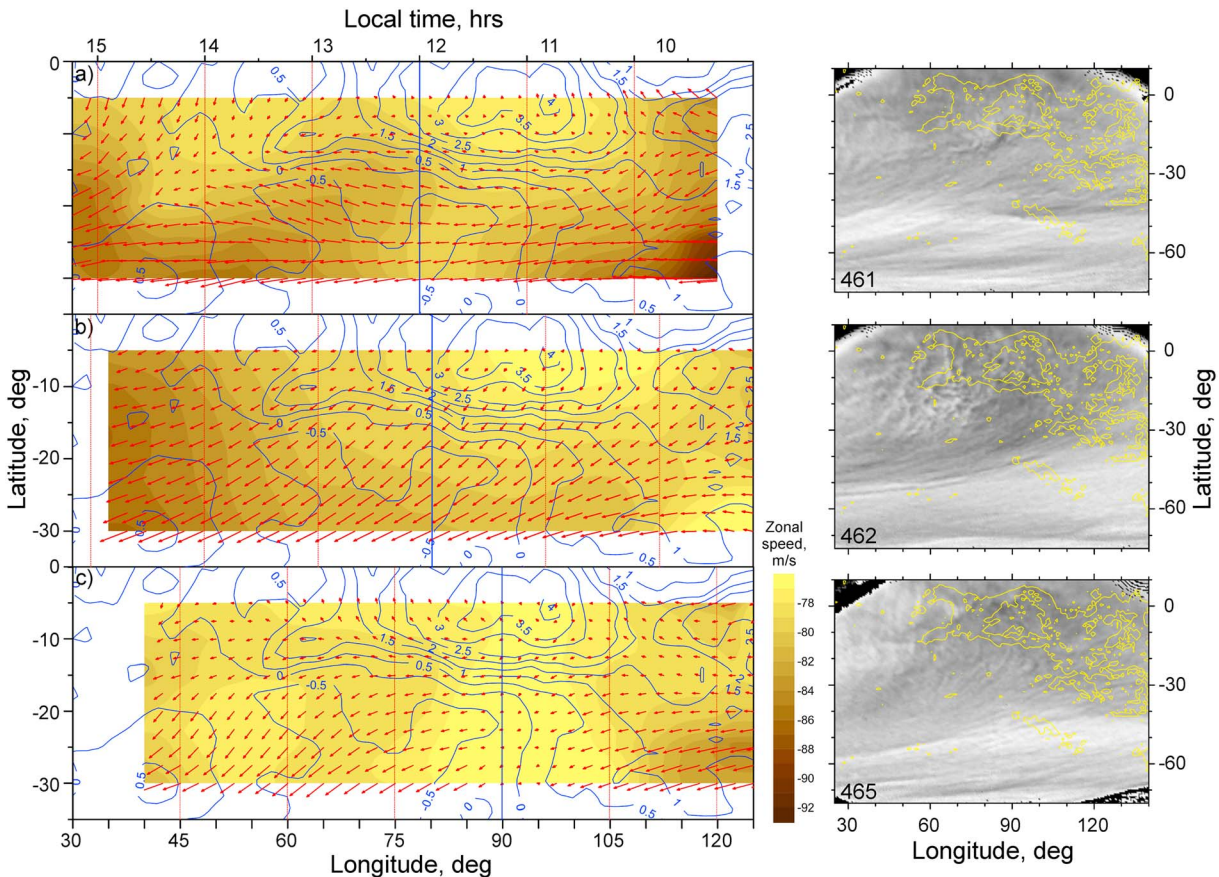
Figure 9. Wind fields for orbits #0461 (a), #0462 (b), and #0465 (c; Tables S12–S14). The results were averaged over [15^\circ\text{E}, 10^\circ\text{S}] bins (longitude, latitude) with a shift of 2.5^\circ in longitude and latitude. Variations of the zonal speed are shown in color. The vectors show the flow direction in a “superrotating” frame. They represent wind velocity after subtraction of the mean zonal speed u_0 \cos(\varphi) where u_0 = -75 m/s and \varphi is latitude. The surface topography is shown as blue contours. Vertical blue lines mark noon. Corresponding UV images in Cartesian projection are shown in the right column.
