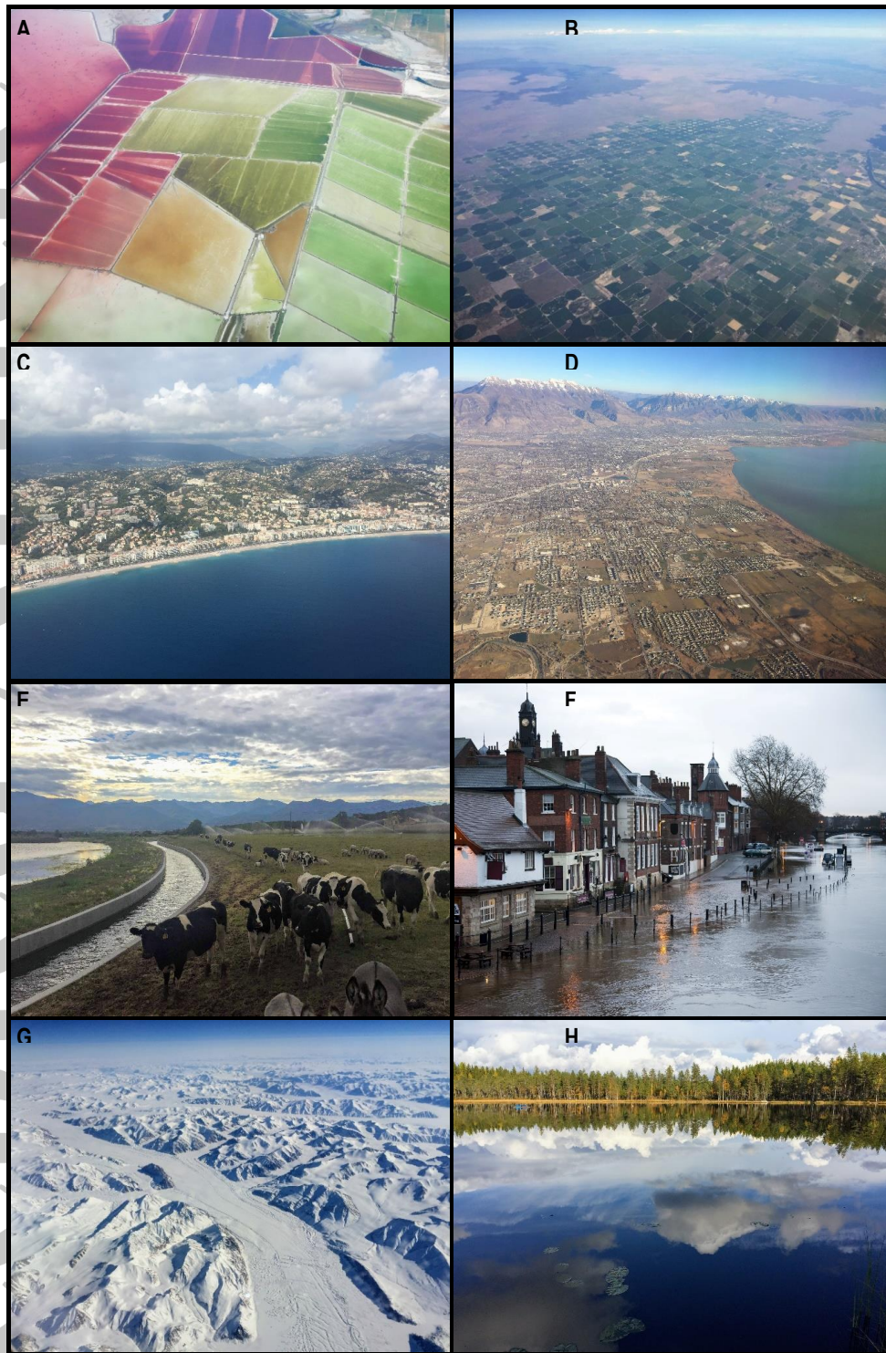
Fig. 2. Photos of human interactions with the water cycle in the Anthropocene. A) Evaporation ponds encroach on the Great Salt Lake, the largest saline lake in the Western Hemisphere, USA; B) Groundwater-fed agriculture and human-caused wildfire, Washington, USA; C) Urban development along the coast in Nice, France. D) Suburban sprawl sustained by inter-basin water transfer around Utah Lake, USA; E) Livestock, canal, and irrigation in Heber City, USA; F) Flooding of the River Ouse in York exceeds defensive engineering infrastructure, UK; G) Accelerating ice discharge from northern Greenland. H) Boreal lake experiencing thermal and chemical modification from atmospheric deposition and climate change, Västerbotten, Sweden.
