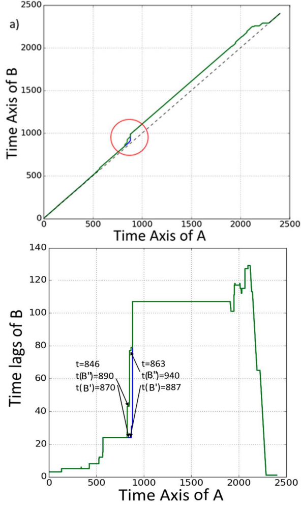
Fig. 7 a In blue, the warping path P_{DTW}(A, B) between the time series A and time series B. In green P_{DTW}(A, B'') the warping path between time series A and time series B'' shown in Fig. 6b. The dashed line represents the diagonal line. b The corresponding time lags.
