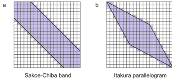
Fig. 3 Examples of global constraints. a Sakoe-Chiba band. b Itakura parallelogram (from Cassisi et al [13])
