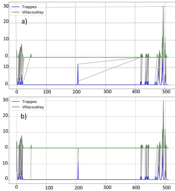
Fig. 5 a FastDTW alignments for two rain gauges time series measured in the cities of Trappes and Villacoublay with a time resolution of T=6 min. The grey lines represent the alignments between the two time series. b Same figure but for IMs-DTW alignments
