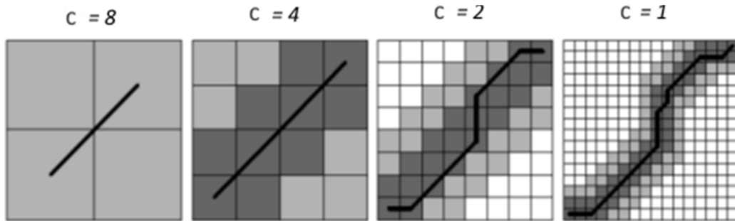
Fig. 4 Illustration of the Salvador et al. algorithm [30]. Dark gray squares are cells that will be evaluated by the constrained DTW. They are derived from the previous step by a “projection” operator. Light grey cells correspond to the released constraint for a radius equal to 1 square. They are also evaluated by the constraint DTW algorithm. White cells are not taken into account by the DTW algorithm. The solid line corresponds to the derived optimal path.
