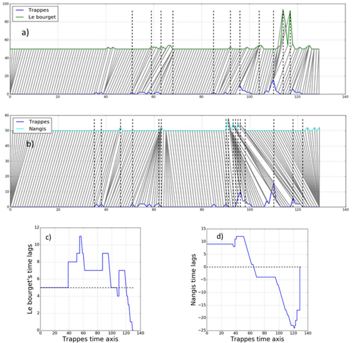
Fig. 10 a warping path for the pair of stations Trappes/ Le Bourget. b warping path for the pair of stations Trappes/Nangis. c the obtained time lags for the pair of station Trappes and Le Bourget. d the obtained time lags for the pair of station Trappes and Nangis
