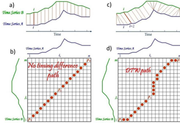
Fig.2 a Comparison between two time series with no timing difference. The grey lines represent the alignments between the two time series. b Warping path associated to a. c Comparison between two time series with some timing differences. d The warping path associated to c (from [23]).
