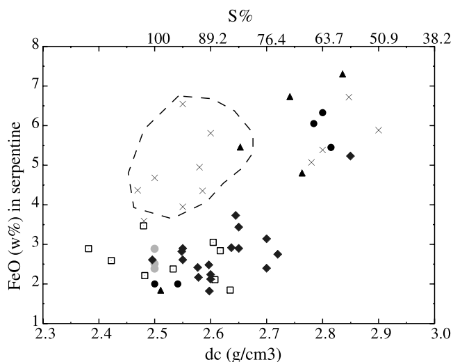
Figure 11. FeO content in serpentine as a function of the corrected grain density ( d_c , proportional to the degree of serpentinization S (in %); see text) in 54 serpentinized peridotite samples from the seven studied drill sites. FeO value for each sample corresponds to the average of 4–14 microprobe measurements. Representative analyses are given in Table 2. High FeO contents in highly serpentinized samples (within dashed line) are attributed to mixture of serpentine with small amounts of iron-brucite and/or iron-oxides (see text). The d_c values <2.515 g/cm 3 , corresponding to 100% serpentinized samples using Miller and Christensen's [1997] empirical formula, in seven samples may be a consequence of porosity, which was not completely saturated during density measurements. Symbols are the same as in Figure 3.
