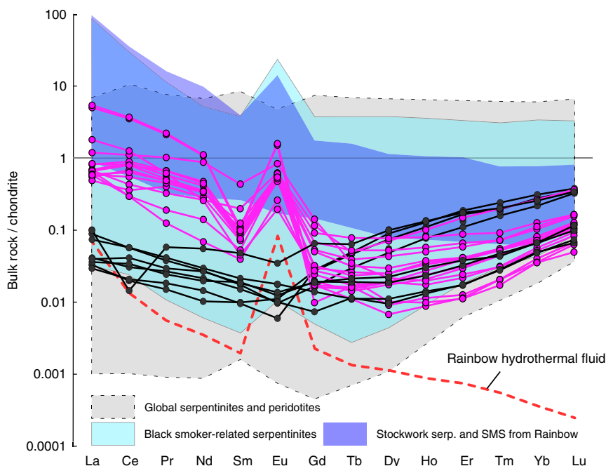
Fig. 1 Chondrite-normalized REE compositions of North Aït Ahmane serpentinites. Hydrothermalized serpentinites (in pink) exhibit significant LREE enrichment and positive Eu anomaly contrasting with unaffected serpentinites (in black). Black smoker fluid of Rainbow (red dotted line) displays the same LREE and Eu pattern despite its lower REE content 19 . Serpentinites and peridotites from abyssal 21,28,61,62 and supra-subduction zone (SSZ) 62–65 settings, black smoker-related serpentinites 21–24 , stockwork serpentinites and semi-massive sulphides from the Rainbow site 23 are shown for comparison. Chondrite normalization values are from Barrat et al. 66
