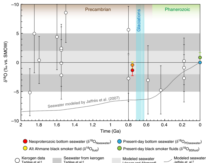
Fig. 7 Oxygen isotopic compositions of the Aït Ahmane hydrothermal fluid and estimate of Neoproterozoic bottom seawater \delta^{18}\text{O} compared with existing estimates along the past 2 Ga. Error bars for \delta^{18}\text{O} values of Aït Ahmane black smoker fluid and Neoproterozoic seawater were calculated following error propagation considering errors on mean \delta^{18}\text{O} value measured on magnetite, on temperature-dependent water-magnetite fractionation and on \Delta^{18}\text{O}_{\text{BSfluid-PDseawater}} ( 2\sigma of the compiled data, Fig. 6), see Supplementary Table 1
