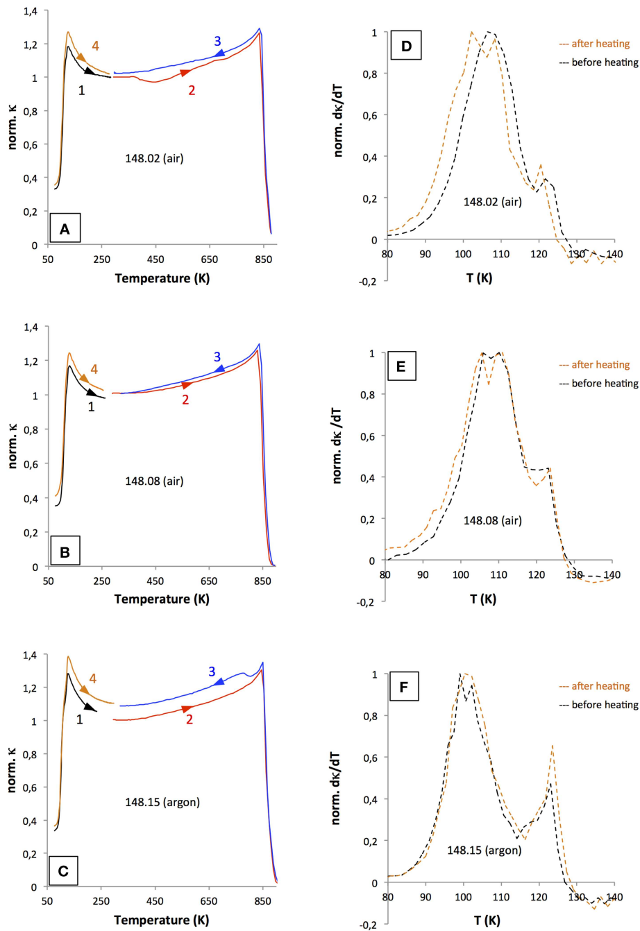
FIGURE 9 | Temperature dependent susceptibility for 148.02 (A), 148.08 (B), and (C) 148.15 experiments performed in air or in argon (data normalized to the room temperature value before heating). Step 1: low temperature measurement from 77
