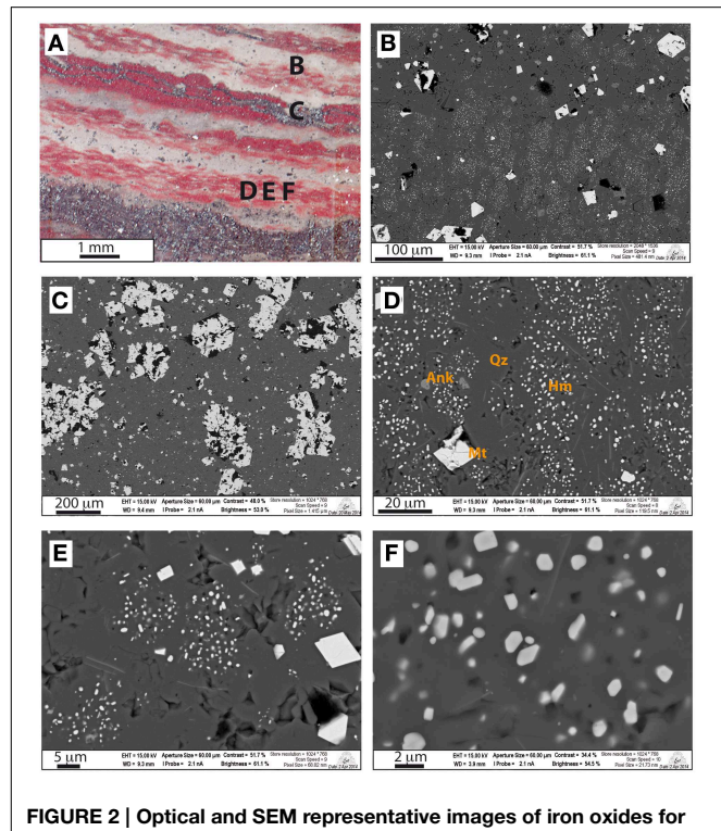
FIGURE 2 | Optical and SEM representative images of iron oxides for sample 130.45. (A) optical microscope image with indications of the area observed with the SEM; (B) SEM image at the transition between gray and red areas; (C) bulky iron oxides within the white gray area interpreted as being magnetite; (D) patches of small euhedral to rounded iron oxide grains interpreted as hematite in the red layers, Qz, quartz; Ank, ankerite; Mt, magnetite; Hm, hematite; (E) small iron oxide grains, interpreted as hematite with bigger grains population interpreted as magnetite and (F) high magnification image of small hematite grains.
